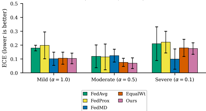
Calibration error by method and non-IID level — PneumoniaMNIST (mean \pm std, 5 seeds)
