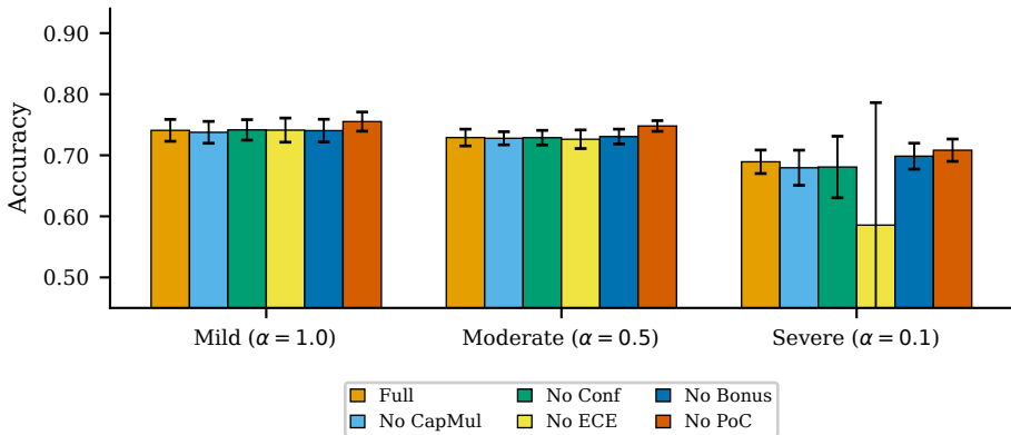
Ablation study — accuracy per component removed — DermaMNIST (mean \pm std, 5 seeds)
