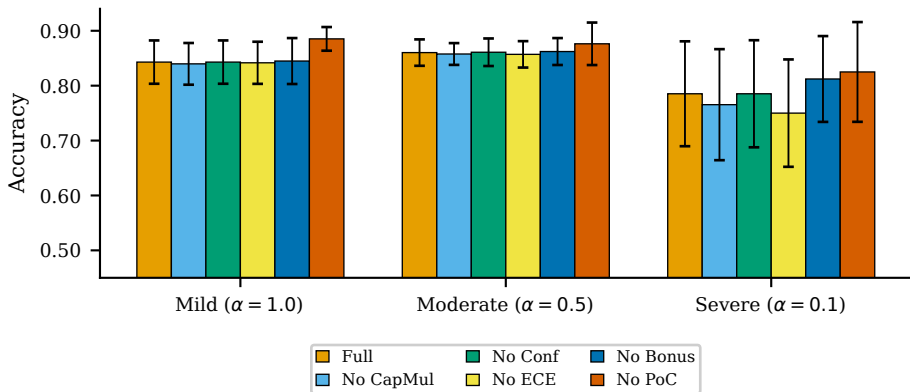
Ablation study — accuracy per component removed — PneumoniaMNIST (mean \pm std, 5 seeds)
