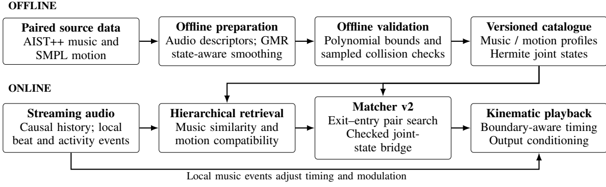
Fig. 1. BeatWeaver overview. Both offline smoothing and online transitions use joint position, velocity, and acceleration. Offline geometric validation does not certify newly synthesized transitions or physical tracking.
