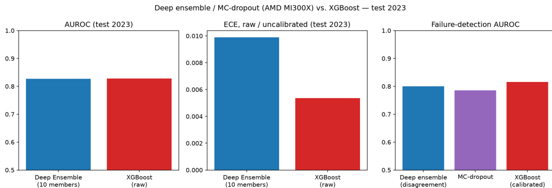
Fig 7: Deep ensemble / MC-dropout (AMD MI300X) vs. XGBoost, test 2023.
