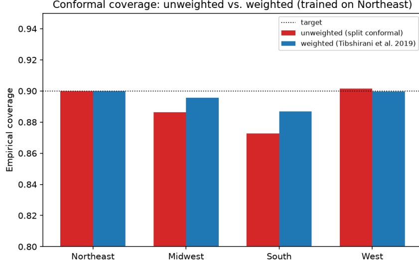
Fig 6: Conformal coverage, unweighted vs. weighted, by region.
