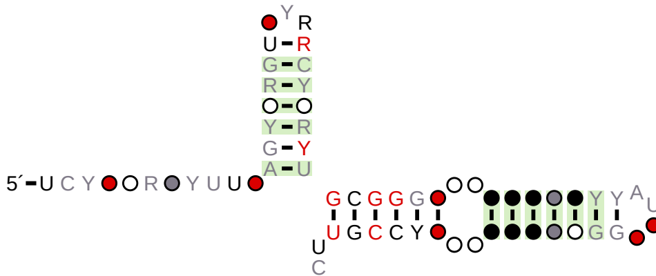
Figure 4: tutorial/updated_Arisong_1.R2R.sto.{pdf,svg} : annotated consensus secondary structure using R2R . Base pairs with covariation scores equal or below the target E-value (0.05 as default) are depicted in green. By default only positions in the alignment with more than 50% occupancy are depicted (unless they form a base pair). Option --r2rall forces the depiction of all positions in the alignment.
