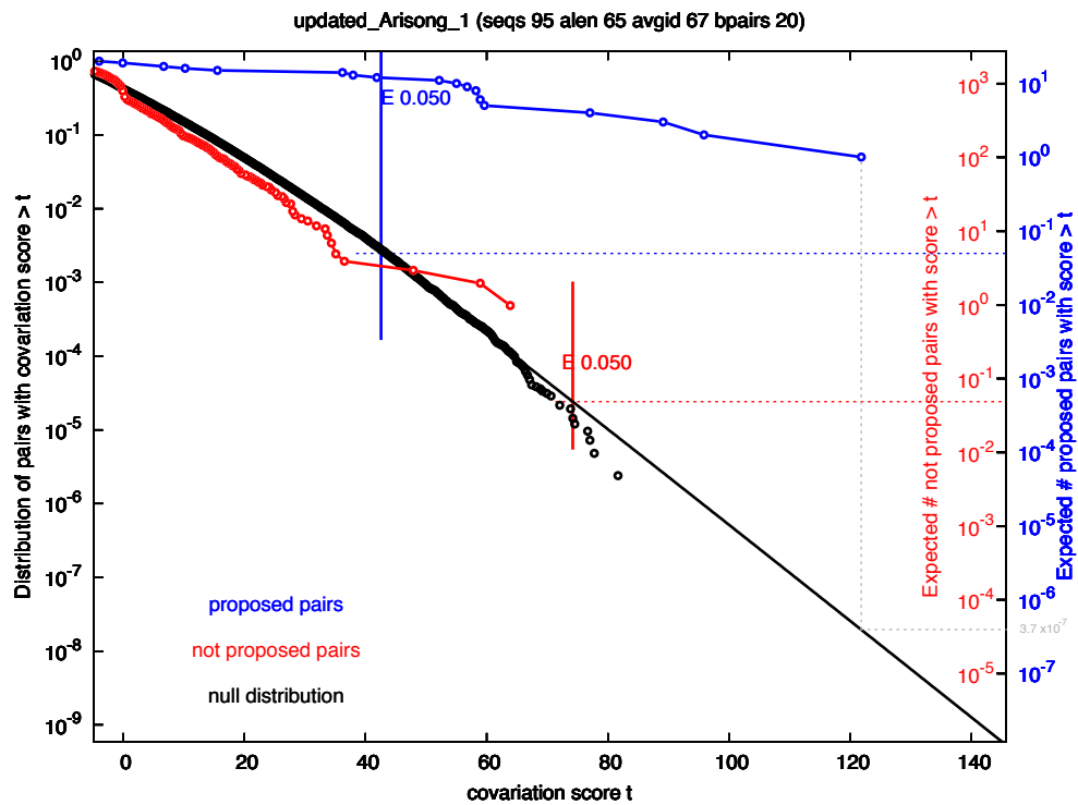
Figure 5: tutorial/updated_Arisong.1.surv.{ps,svg} : covariation scores survival function P(X > x) . The survival function of scores for all pairs in the given alignment is depicted in blue. The survival function for the null alignments is depicted in black. A black line indicates to fit to a truncated Gamma distribution of the tail of the null distribution. In red, we plot the survival function of scores for the pairs in the given alignment excluding those proposed as base pairs. For a particular pair, as an example the highest scoring one from the distribution of proposed pairs (blue), we obtain its E-value by drawing a vertical (gray) line from the point to the null distribution (black). The corresponding value in the blue scale gives us the E-value for that pair (in this example, 3.7 \cdot 10^{-7} ).
