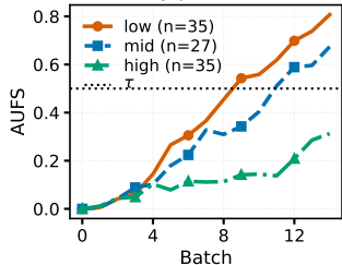
AUFS by pretest bucket
