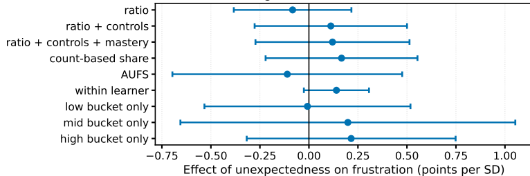
(b) Regression estimates with 95% CI
