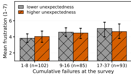
(a) Same failures, different unexpectedness (pooled difference -0.08 [-0.65, +0.52])
