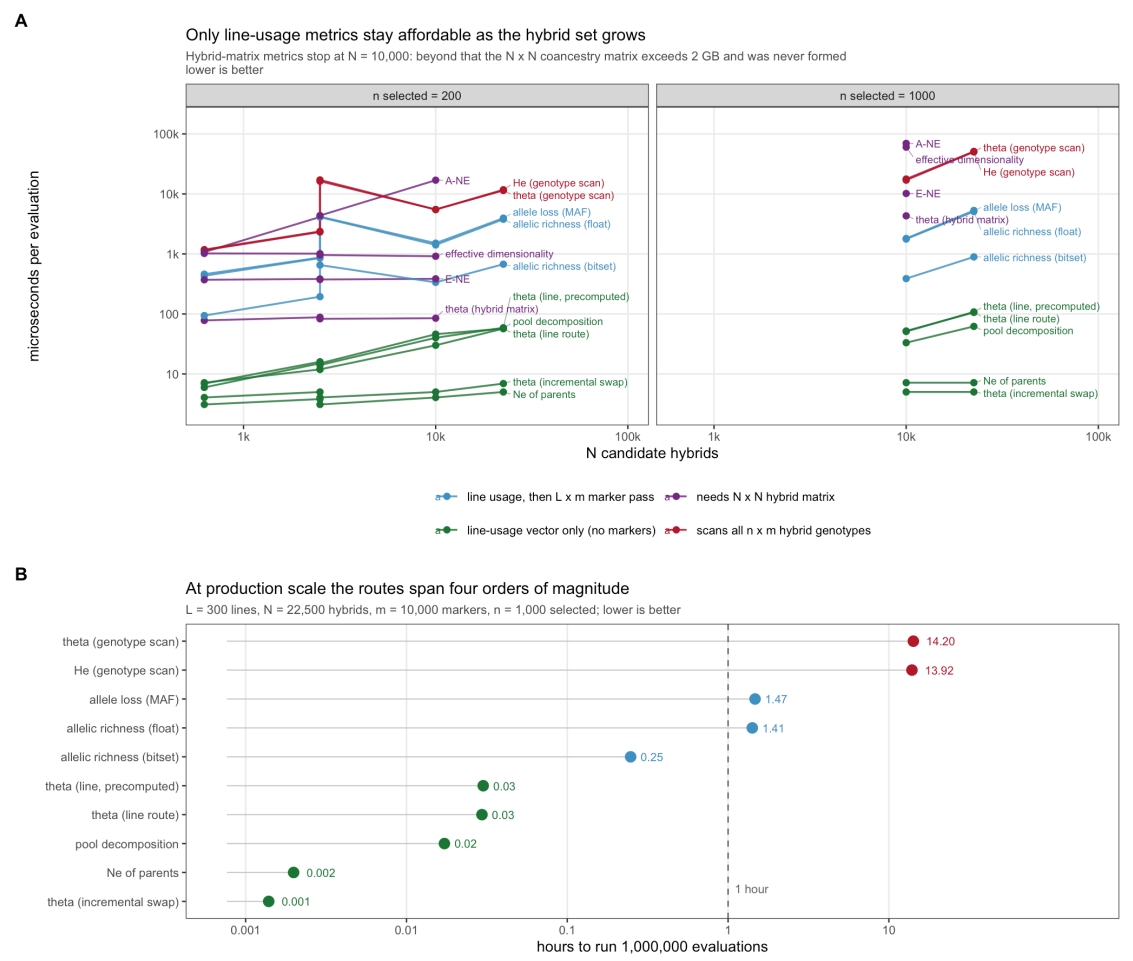
Figure 11.1: Cost per fitness evaluation. Panel A: scaling in the number of candidate hybrids. Panel B: hours to complete one million evaluations at production scale.
