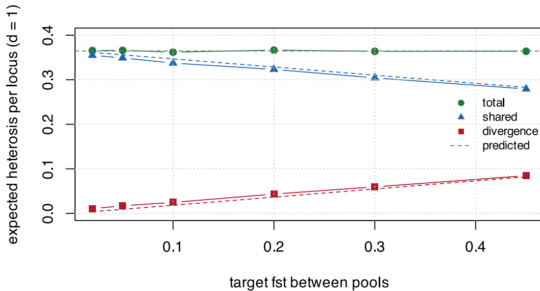
Figure 9.1: Expected heterosis and its two components as the pools are driven apart by drift alone. Dashed lines are the Balding-Nichols predictions for each component separately, with no fitted parameter. The divergence term grows eightfold; the shared term pays for all of it, unit for unit; the total is flat. Nothing is selected here – this is what neutral divergence does.
