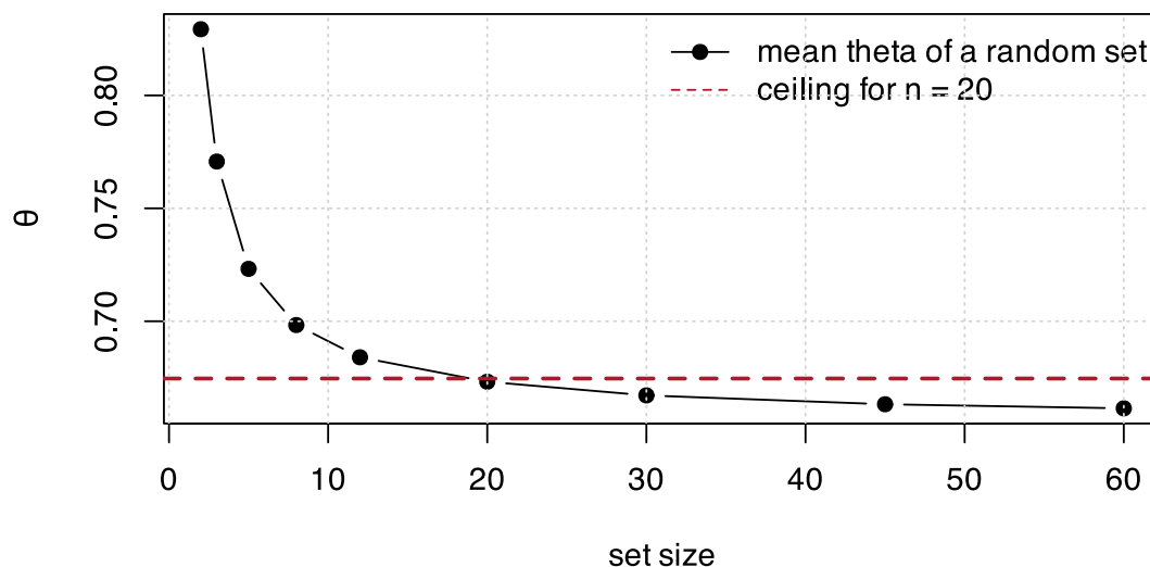
Figure 12.2: Group coancestry falls monotonically with set size. A ceiling calibrated at the target size is unreachable at every smaller size, which is why an incremental greedy stops at the first candidate.
