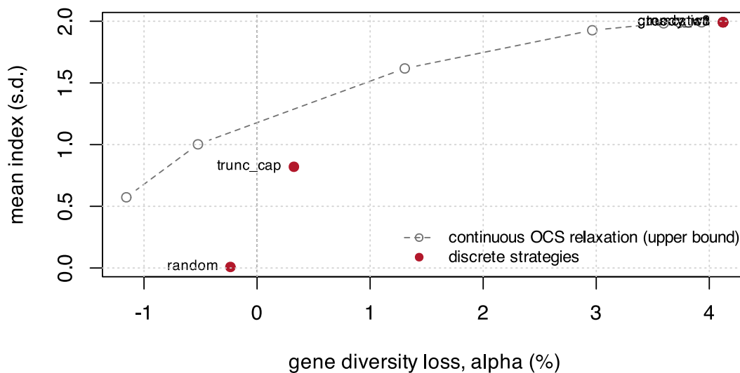
Figure 14.1: The continuous relaxation traces an upper bound. Discrete strategies must sit below and to the left of it; how far below is the convergence diagnostic.
