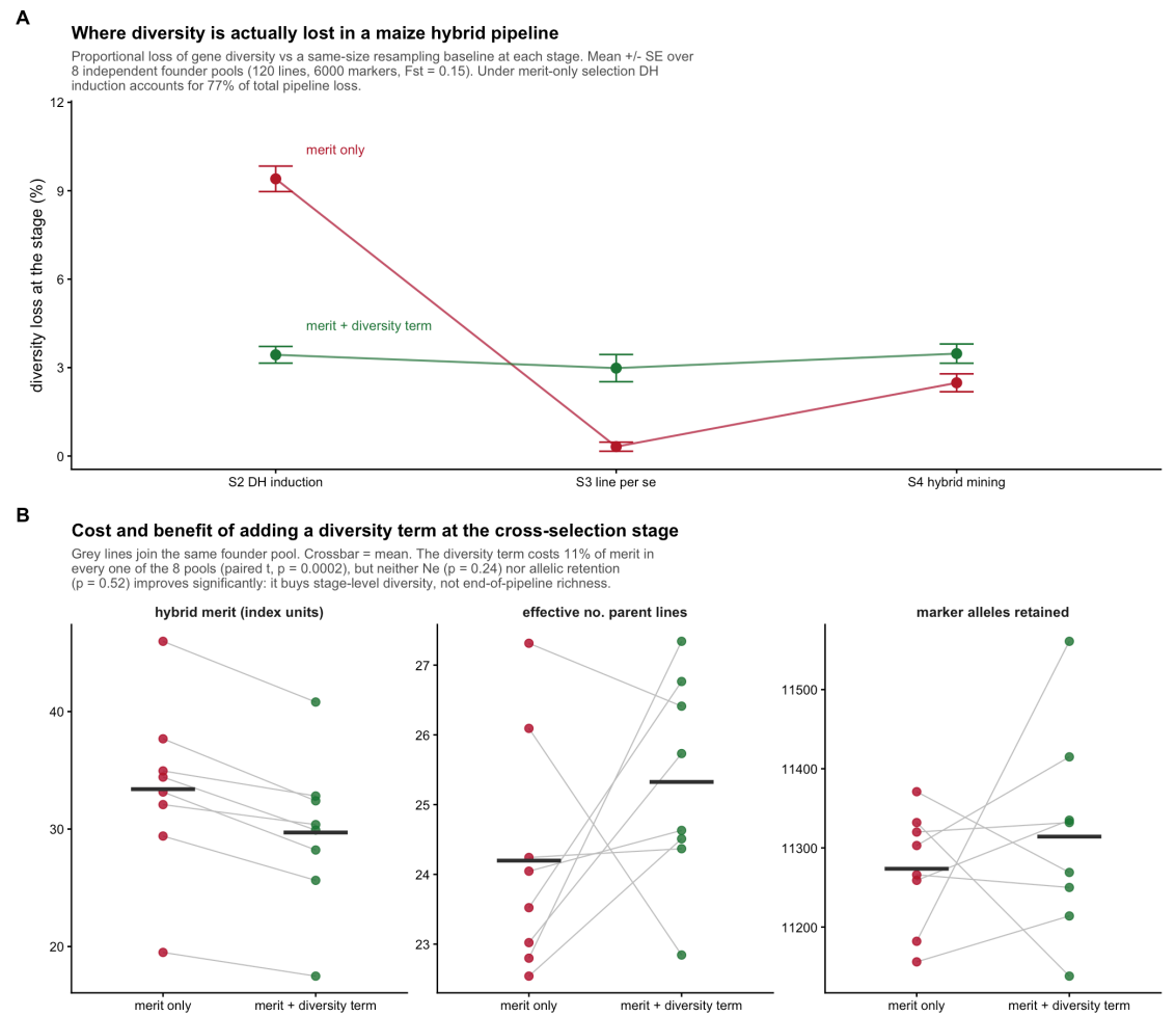
Figure 12.3: Where the diversity goes. DH induction dominates, and a diversity term applied there redistributes loss rather than removing it.
