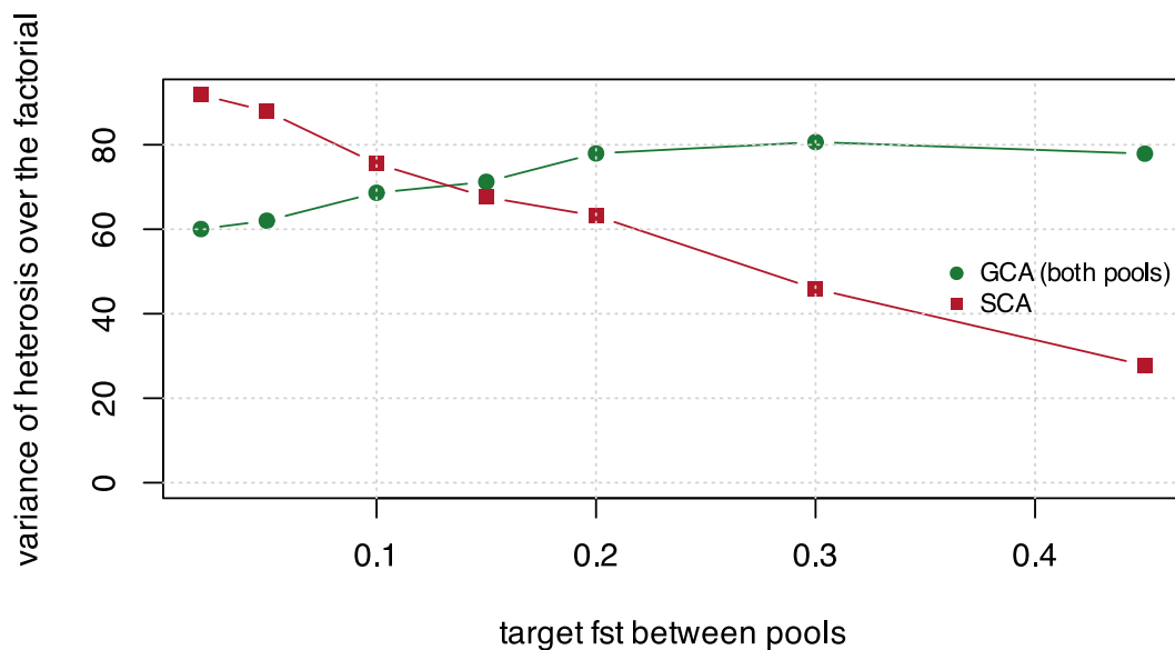
Figure 9.3: The same neutral divergence sweep, read through the combining-ability decomposition rather than through the mean. Expected heterosis is flat across this entire range (previous figure); its decomposition is not. Specific combining ability falls by two thirds while general combining ability rises, so the share of hybrid variation that is specific drops from about 0.60 to 0.26. Divergence does not create heterosis – it moves heterosis into the half of the model an additive predictor can express.
