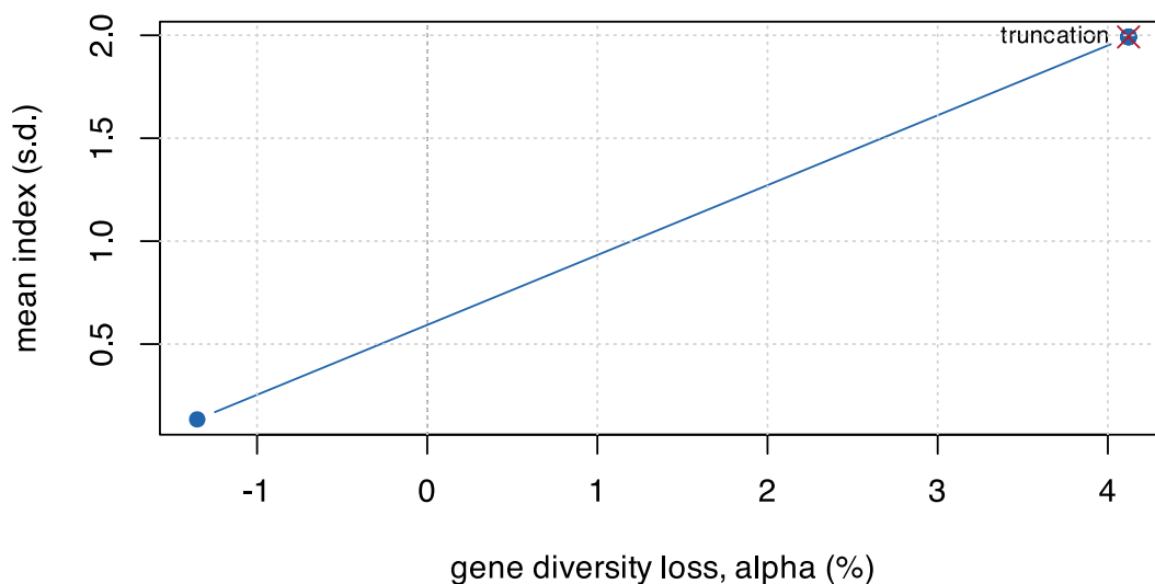
Figure 15.1: The greedy frontier. w = 0 is maximum diversity; large w converges to truncation.
