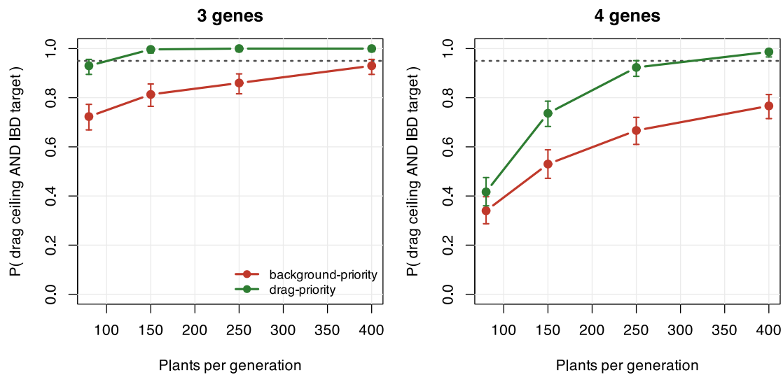
Figure 6.2: Paired comparison (common random numbers, 300 replicates, s = 0.60 ) of the two-stage background-priority index against the drag-priority index. Bars are Clopper-Pearson 95% intervals. The criterion is drag \leq 30 cM per gene AND IBD \geq 0.90 at BC3.
