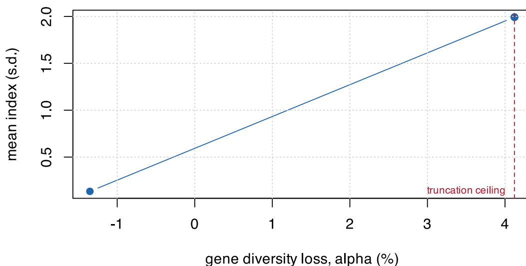
Figure 14.2: The greedy frontier, swept over the merit weight w . The knee is where further diversity costs index steeply.
