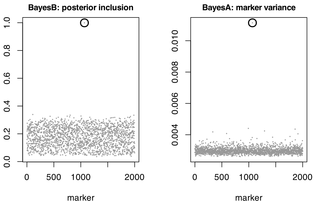
Figure 13.1: The two priors on the same oligogenic trait, with the marker carrying 96% of the genetic variance circled. Both find it. Only BayesB can then remove the other 1999 from the model.
