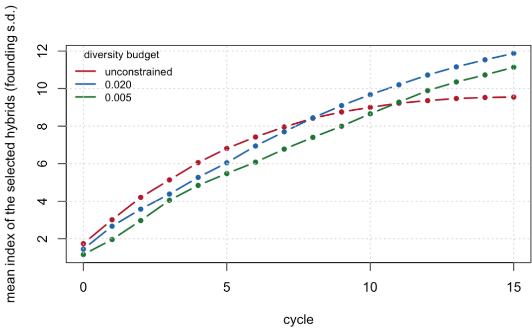
Figure 18.2: Mean index of the selected hybrids, in founding-cycle standard deviations, averaged over five seeds. The unconstrained programme leads for eight cycles and then stops climbing. Neither constrained programme has stopped by cycle 15.
