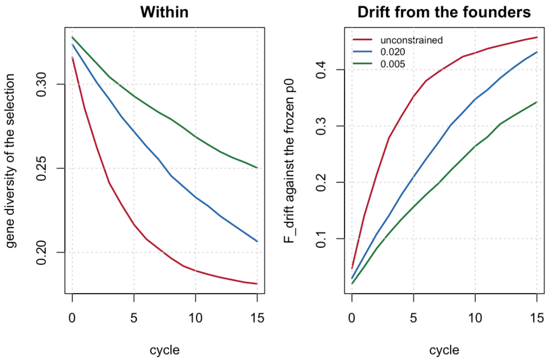
Figure 18.3: Left: gene diversity of the selection. Right: F_{\text{drift}} against the frozen founding base. The unconstrained programme spends nearly its whole diversity endowment by cycle 8 and has little left to convert afterwards.
