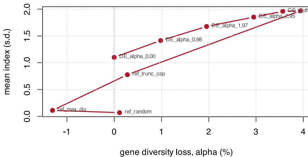
Figure 21.1: The price list. Each point is one diversity budget; the curve is what index it buys.
