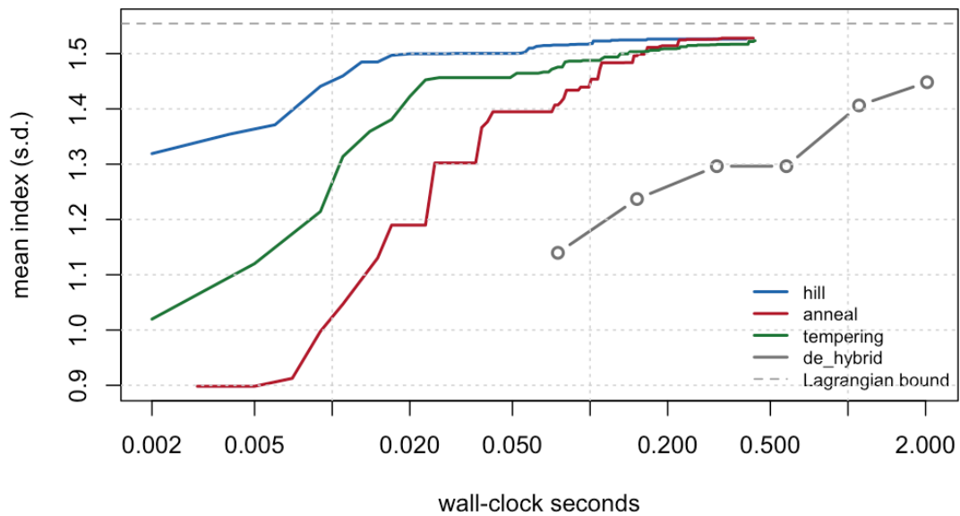
Figure 17.1: Best index reached against wall-clock seconds, at book scale under a 1% diversity budget. The dashed line is the Lagrangian bound of Section 17.4. Local search is at 1.52 within a tenth of a second; the differential evolution reaches only 1.45 after two seconds.
