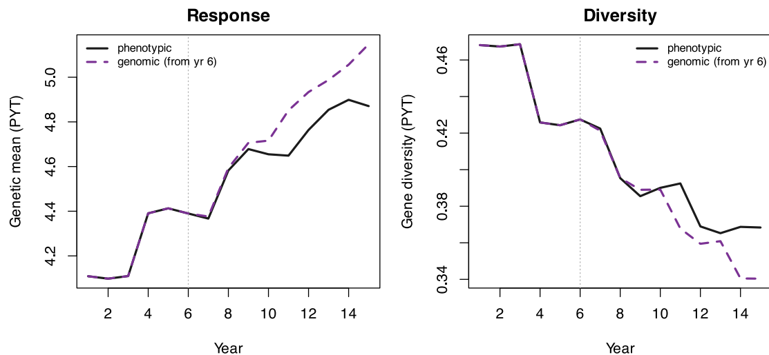
Figure 8.2: Twenty-four paired runs, genomic selection switched on in year 6. Left: genetic mean of the preliminary yield trial. Right: gene diversity of the same population. The faster programme is also the one spending diversity faster.
