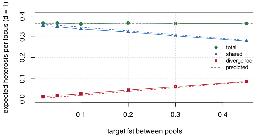
Figure 10.1: Expected heterosis and its two components as the pools are driven apart by drift alone. Dashed lines are the Balding-Nichols predictions for each component separately, with no fitted parameter. The divergence term grows eightfold; the shared term pays for all of it, unit for unit; the total is flat. Nothing is selected here – this is what neutral divergence does.
