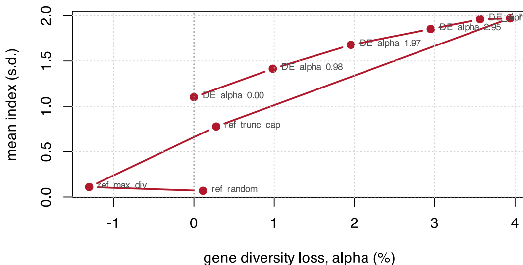
Figure 21.1: The price list. Each point is one diversity budget; the curve is what index it buys.
