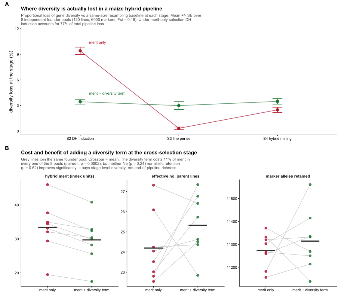
Figure 13.3: Where the diversity goes. DH induction dominates, and a diversity term applied there redistributes loss rather than removing it.
