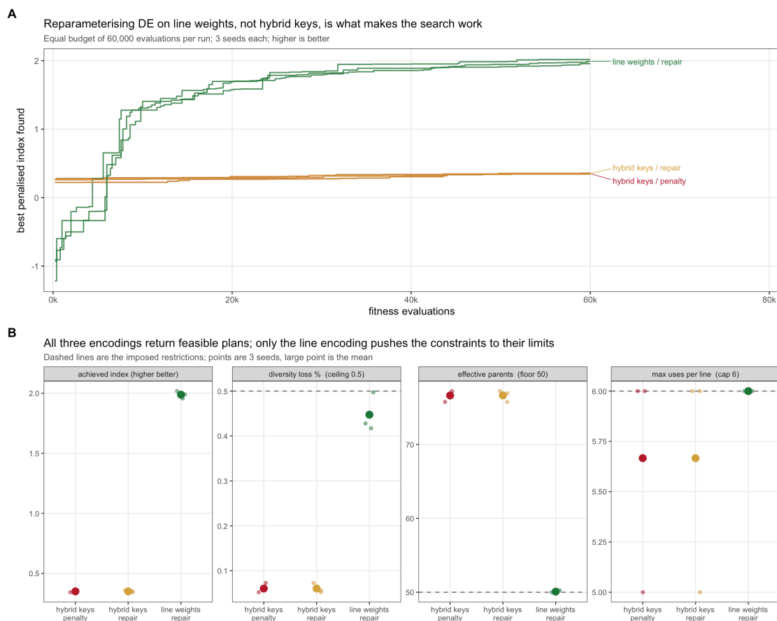
Figure 10.4: Differential evolution under four simultaneous restrictions at equal evaluation budget.
