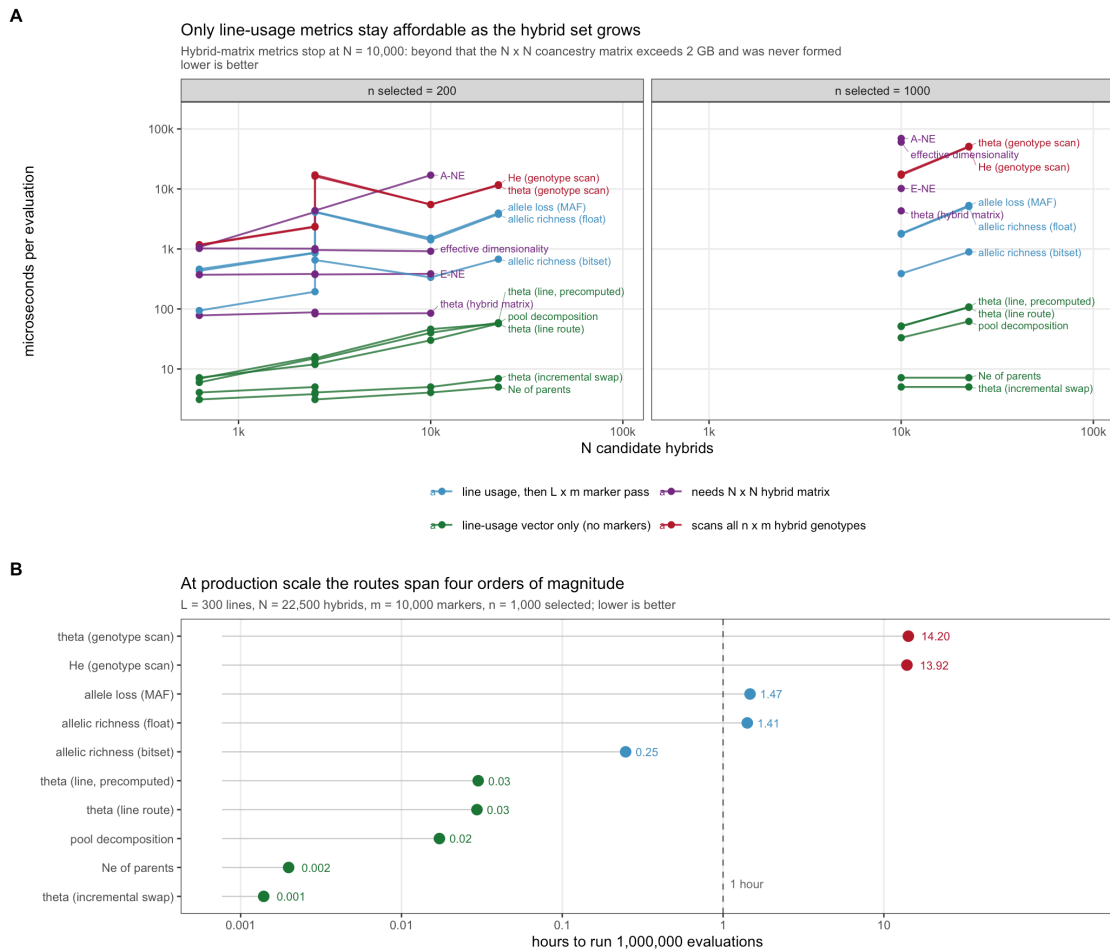
Figure 9.1: Cost per fitness evaluation. Panel A: scaling in the number of candidate hybrids. Panel B: hours to complete one million evaluations at production scale.
