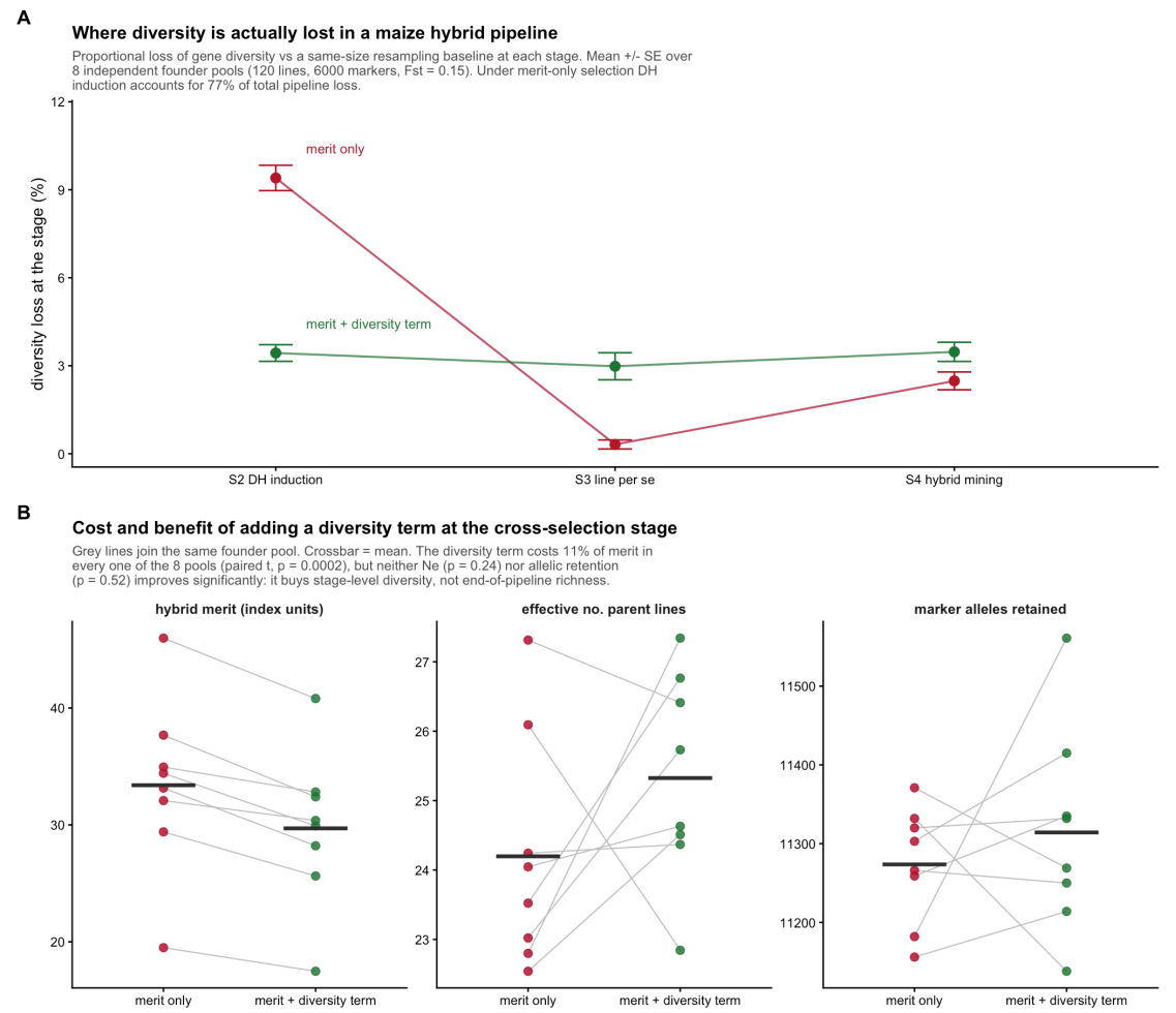
Figure 10.3: Where the diversity goes. DH induction dominates, and a diversity term applied there redistributes loss rather than removing it.
