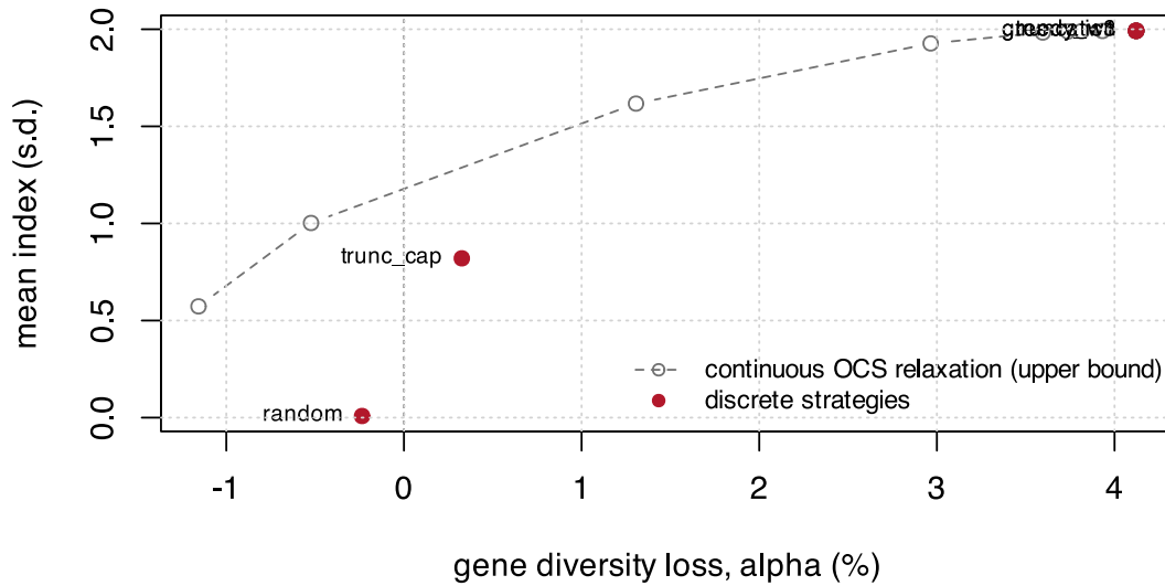
Figure 11.1: The continuous relaxation traces an upper bound. Discrete strategies must sit below and to the left of it; how far below is the convergence diagnostic.
