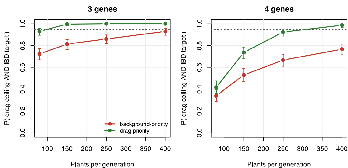
Figure 5.2: Paired comparison (common random numbers, 300 replicates, s = 0.60 ) of the two-stage background-priority index against the drag-priority index. Bars are Clopper-Pearson 95% intervals. The criterion is drag \leq 30 cM per gene AND IBD \geq 0.90 at BC3.
