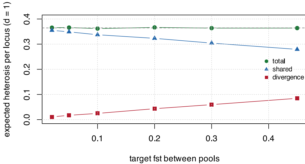
Figure 7.1: Expected heterosis and its two components as the pools are driven apart by drift alone. The divergence term grows eightfold; the shared term pays for all of it; the total is flat. Nothing is selected here – this is what neutral divergence does.
