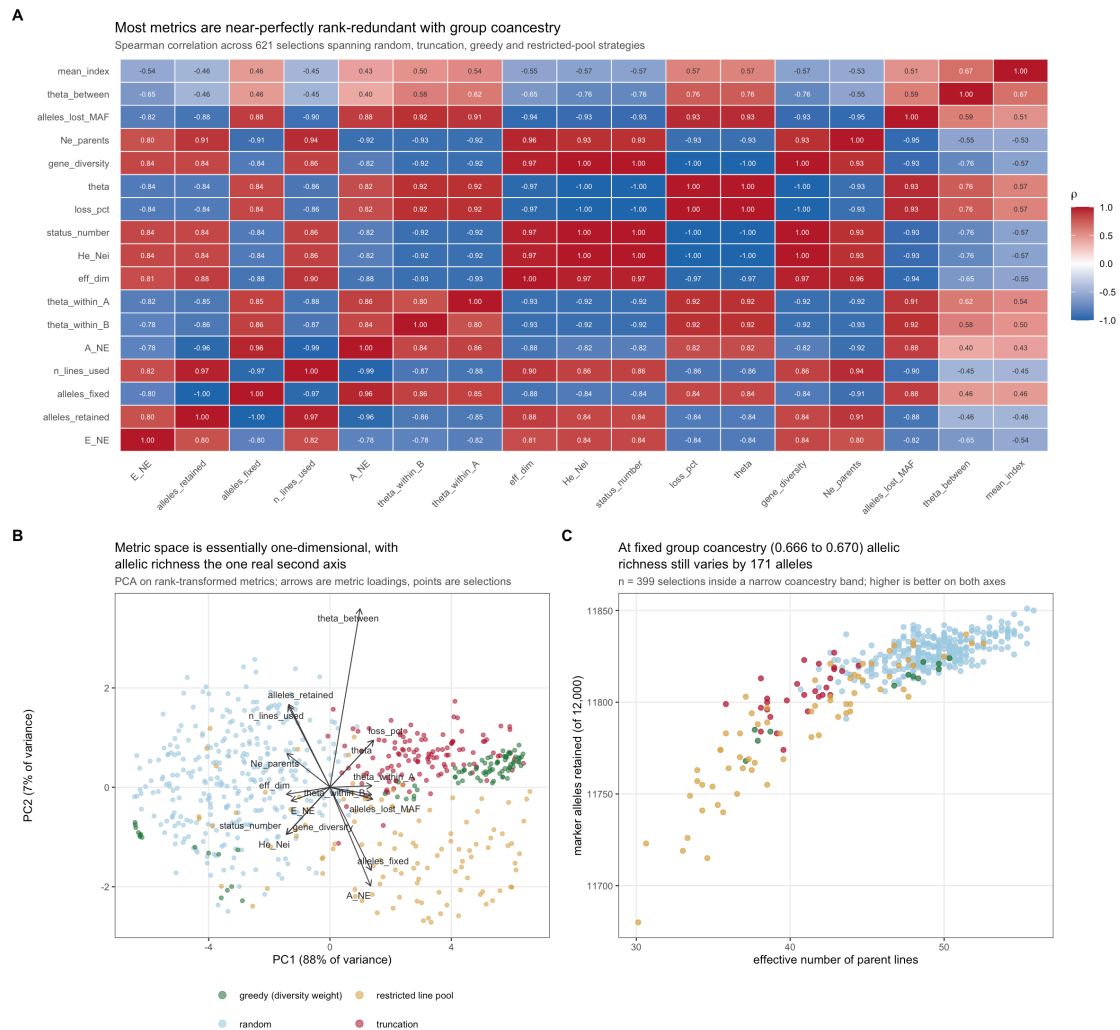
Figure 7.2: Metric redundancy. A: Spearman correlations. B: PCA of rank-transformed metrics. C: the discriminating case, inside a narrow coancestry band.
