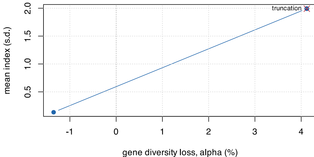
Figure 10.1: The greedy frontier. w = 0 is maximum diversity; large w converges to truncation.
