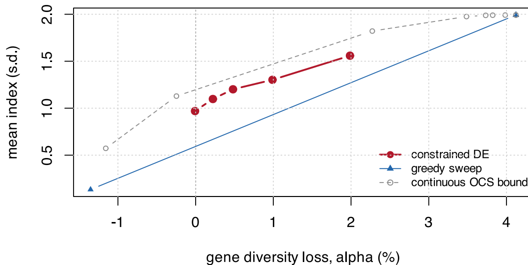
Figure 10.3: Everything together. The constrained DE, the greedy sweep, the continuous upper bound, and the fixed reference strategies.
