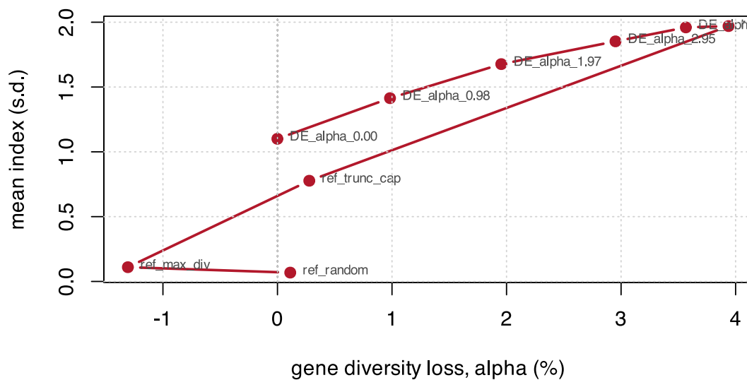
Figure 12.1: The price list. Each point is one diversity budget; the curve is what index it buys.
