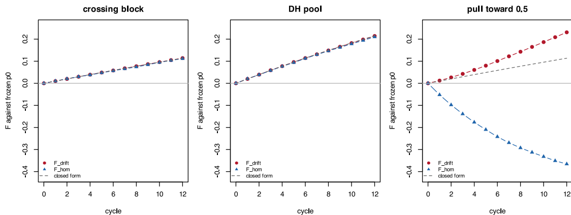
Figure 9.1: The two lenses on one heterotic pool over 12 cycles, averaged over 20 replicates, against a base frozen at cycle 0. Left: a crossing block of 50 plants (100 gametes per cycle). Centre: the same 50 lines re-derived as doubled haploids (50 allele copies per cycle), which drifts at twice the rate. In both, the closed form 1 - (1 - 1/n_{\text{gam}})^t is the dashed line and the two lenses sit on it. Right: the crossing block with every frequency moved 5% toward 0.5 before each drift step, where the homozygosity lens reports a gain of heterozygosity against the frozen base while the drift lens reports more than twice the neutral rate; the dashed line is the same neutral closed form, here a reference both lenses leave. Nothing is selected in any panel; the divergence in the right-hand panel is produced by the management rule alone.
