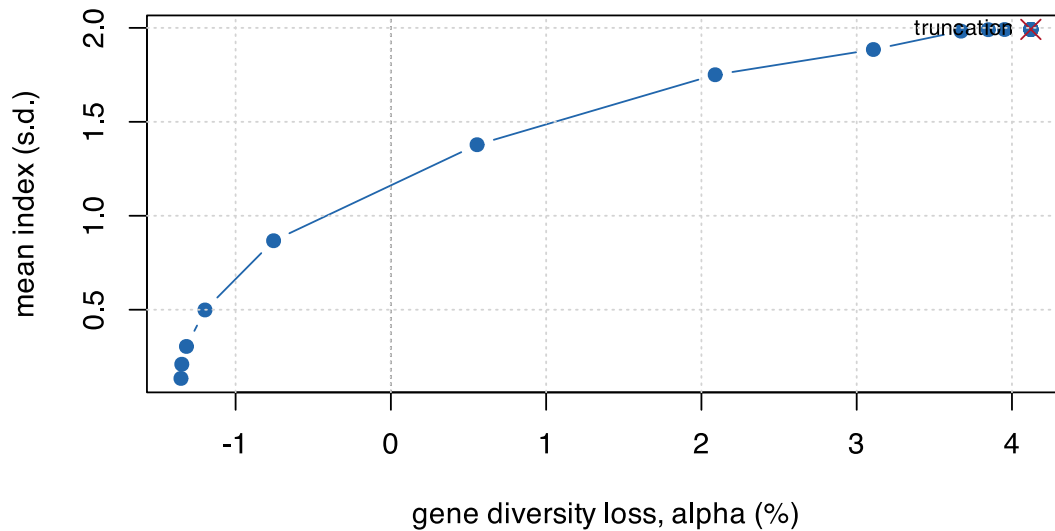
Figure 16.1: The greedy frontier. w = 0 is maximum diversity; large w converges to truncation. The useful range of w spans roughly 1e-5 to 1e-2 on this dataset, the same window the prose and the sweep table below quote: below it the sweep returns the maximum-diversity plan, above it the truncation plan, and every row outside the window is a duplicate of one of those two.
