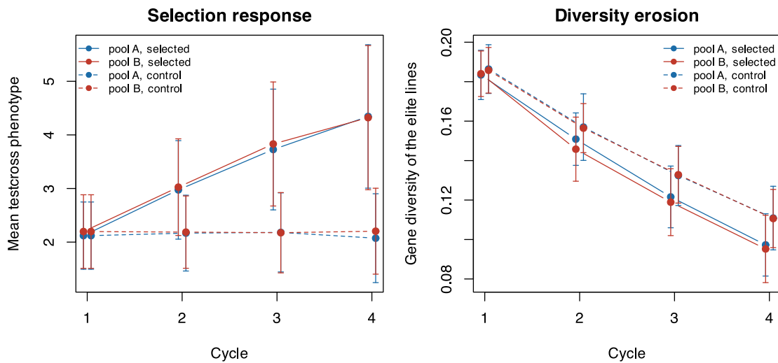
Figure 7.1: Reciprocal recurrent selection over 4 cycles at book scale, 48 founder draws, selection (solid) against the paired no-selection control (dashed); points are means over draws and bars one standard deviation. Left: mean testcross phenotype per pool, measured on all DH lines tested that cycle. Right: gene diversity of the elite lines retained each cycle.
