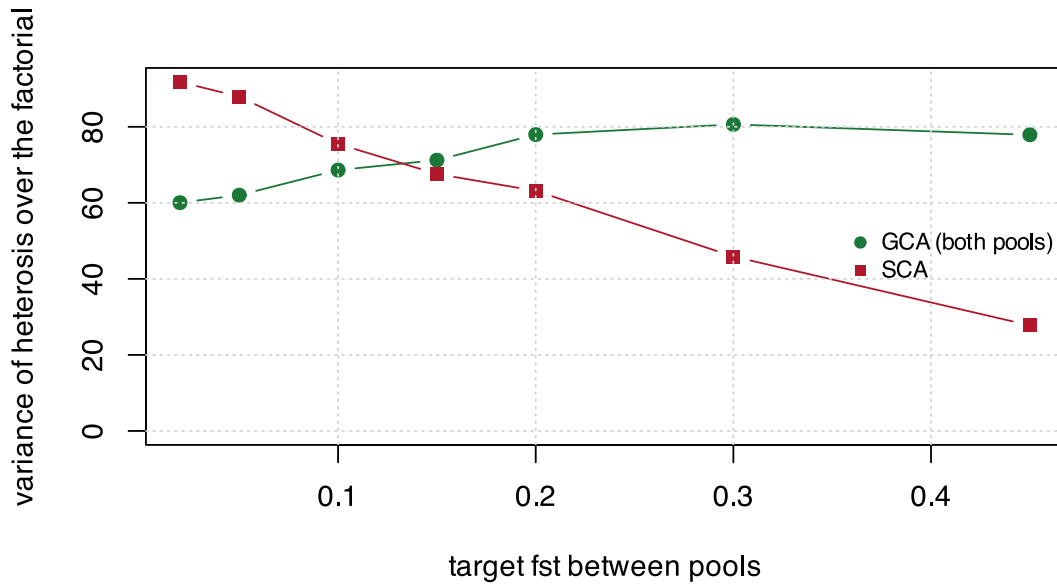
Figure 10.3: The same neutral divergence sweep, read through the combining-ability decomposition rather than through the mean. Expected heterosis is flat across this entire range (Figure 10.1); its decomposition is not. Specific combining ability falls steeply throughout. General combining ability rises, by much less than SCA loses, and itself turns over inside the range – both components vanish at F_{ST} = 1 . The two curves do not sum to a constant: most of the SCA variance lost is destroyed rather than relocated, and the exact percentages are in the text.
