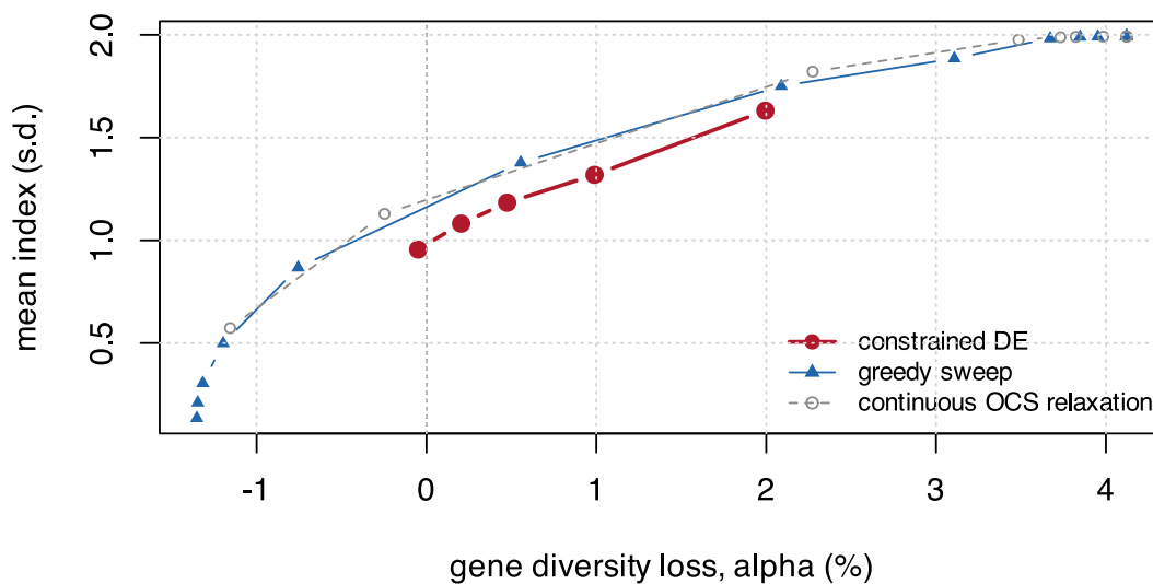
Figure 16.3: Everything together. The constrained DE, the greedy sweep, and the continuous OCS relaxation – which is a relaxation, not a bound at matched diversity (Section 17.4).
