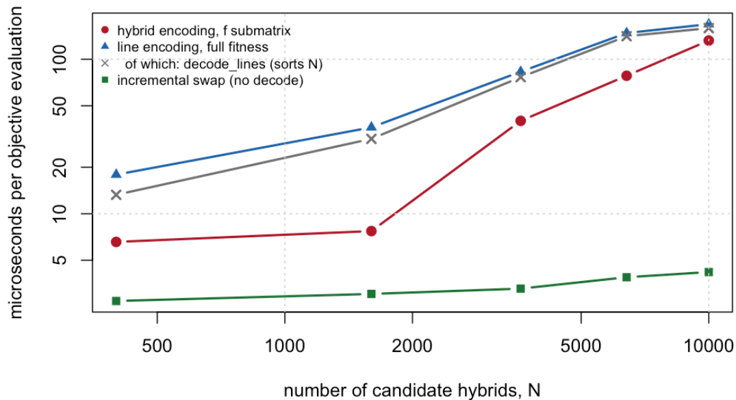
Figure 17.2: Cost per objective evaluation against the number of candidate hybrids. Only the incremental swap is flat. Both encodings grow: the line route by 9.4x, dominated by decode_lines() 's O(N \log N) sort over all candidates, and the hybrid route by 20x – but that arm is confounded, because the sweep sets n_sel to 2 percent of N (20 crosses at N = 400, 200 at N = 10,000) and \text{mean}(f[\text{idx}, \text{idx}]) is quadratic in the selection, not in N .
