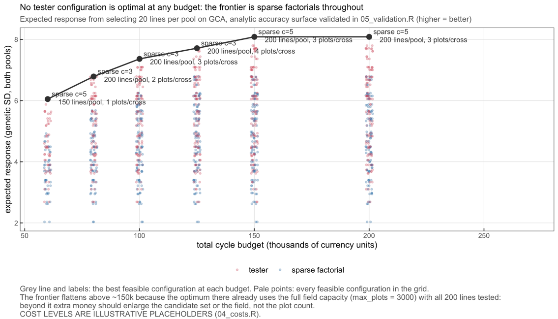
Figure 9.7: The optimiser’s budget frontier. Cached from the sparsex optimiser.
