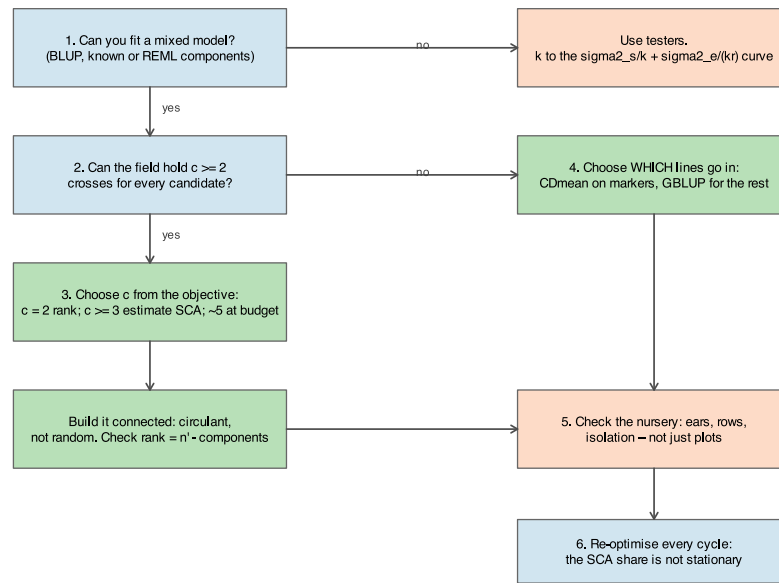
Figure 9.8: A decision procedure for the crossing plan of a two-pool programme. Each question is answered by a section of this chapter.
