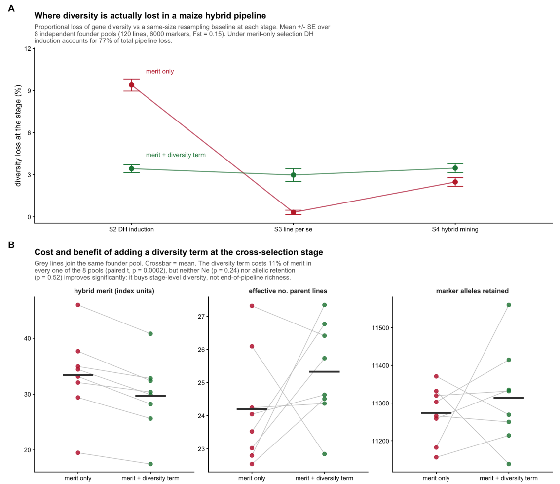
Figure 14.3: Where the diversity goes. DH induction dominates, and a diversity term applied there redistributes loss rather than removing it.
