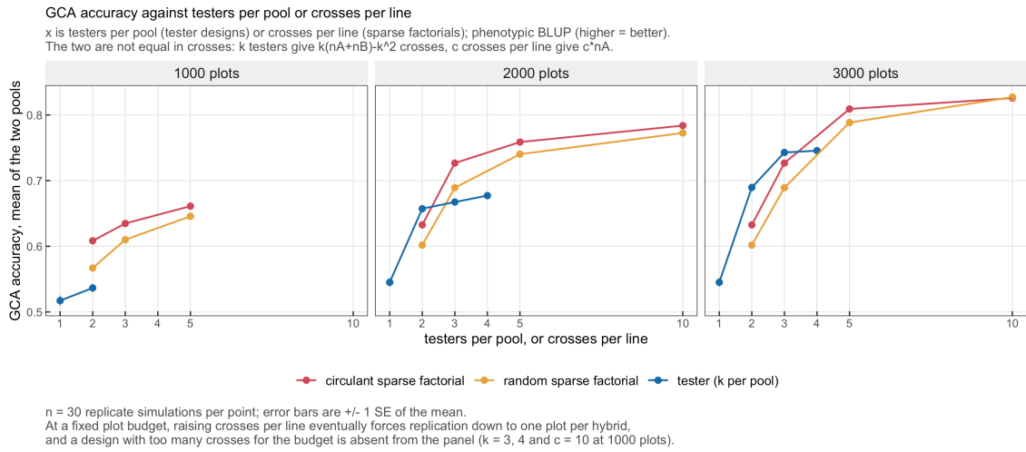
Figure 9.4: GCA accuracy against crosses per line c , separating circulant (structured) from random sparse layouts. Cached from the sparsesex sweep.
