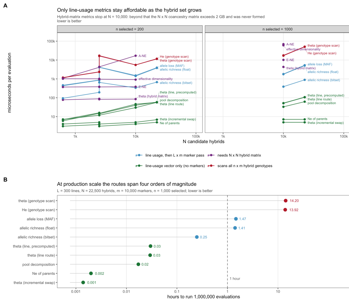
Figure 13.1: Cost per fitness evaluation. Panel A: scaling in the number of candidate hybrids. Panel B: hours to complete one million evaluations at production scale.
