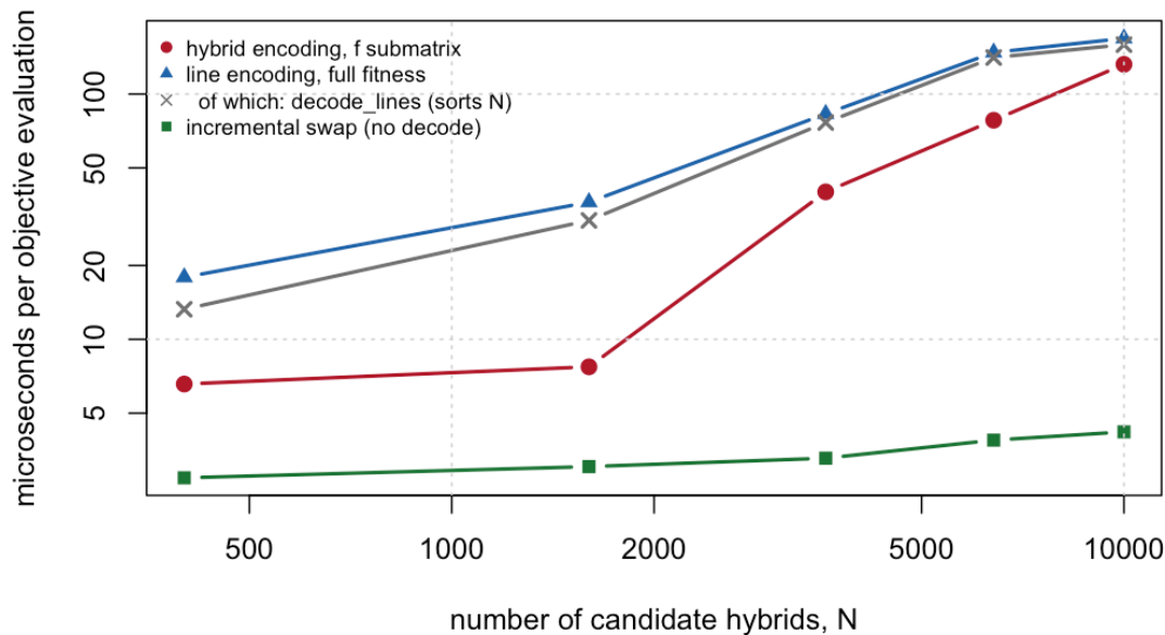
Figure 18.2: Cost per objective evaluation against the number of candidate hybrids. Only the incremental swap is flat. Both encodings grow: the line route by 9.4x, dominated by decode_lines() 's O(N \log N) sort over all candidates, and the hybrid route by 20x – but that arm is confounded, because the sweep sets n_sel to 2 percent of N (20 crosses at N = 400, 200 at N = 10,000) and mean(f[idx, idx]) is quadratic in the selection, not in N .
