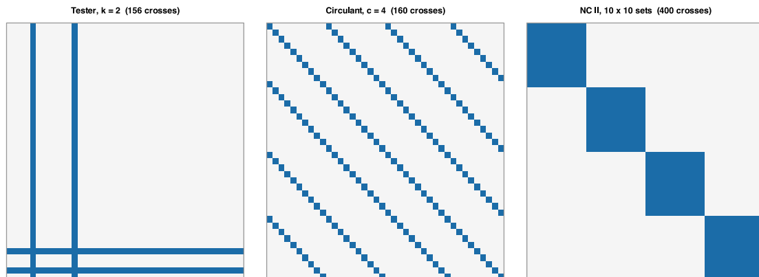
Figure 9.1: Three samples of the same 40 x 40 factorial, drawn by the package's own generators. Rows are pool-A lines, columns pool-B lines, a filled cell is a cross that goes to the field. Left: two testers per pool (156 crosses). Centre: a circulant sparse factorial with four crosses per line (160 crosses). Right: North Carolina Design II as four disconnected 10 x 10 blocks (400 crosses).
