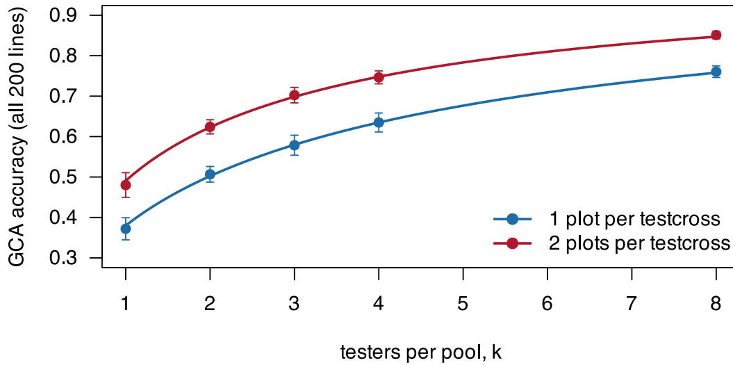
Figure 9.2: GCA accuracy of a k -tester design against the number of testers, at one and two plots per testcross. Lines: the closed form of Table 9.1. Points: least-squares estimates from fit_gca() on the 200 x 200 running example, mean of 12 replicates with the truth redrawn each time; bars are two standard errors.
