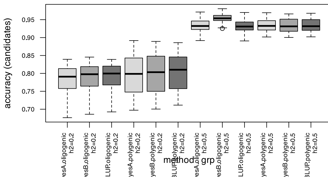
Figure 15.2: Prediction accuracy by architecture and heritability, 15 replicate splits each.
