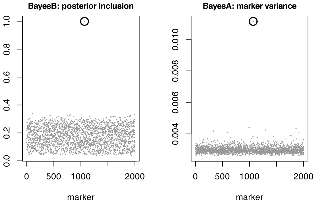
Figure 15.1: The two priors on the same oligogenic trait, with the marker carrying 96% of the genetic variance circled. Both find it. Only BayesB can then remove the other 1999 from the model.
