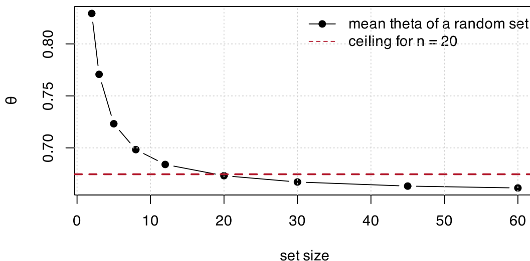
Figure 14.2: Group coancestry falls monotonically with set size. A ceiling calibrated at the target size is unreachable at every smaller size, which is why an incremental greedy stops at the first candidate.
