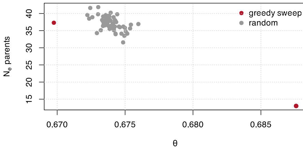
Figure 13.3: At fixed theta, the effective number of parents still varies by a factor of two. The constraint cannot see the difference; the second metric can.
