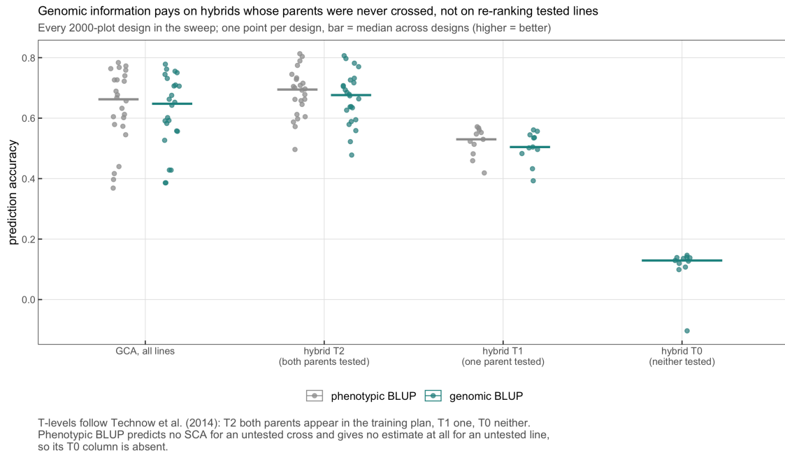
Figure 9.5: Genomic against phenotypic BLUP by design (left) and the genomic accuracy for hybrids whose parents were never crossed (right). Cached from the sparsex sweep, 2,000 plots.
