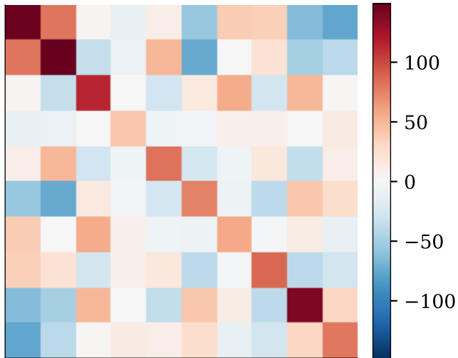
Generated SPD matrix A
