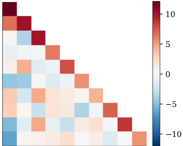
Cholesky factor G
