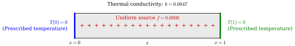
Figure 2: One-dimensional steady-state heat-conduction configuration for the generated Dirichlet–Dirichlet boundary conditions.
