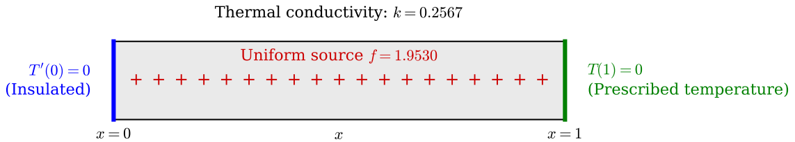
Figure 2: One-dimensional steady-state heat-conduction configuration for the generated Neumann–Dirichlet boundary conditions.
