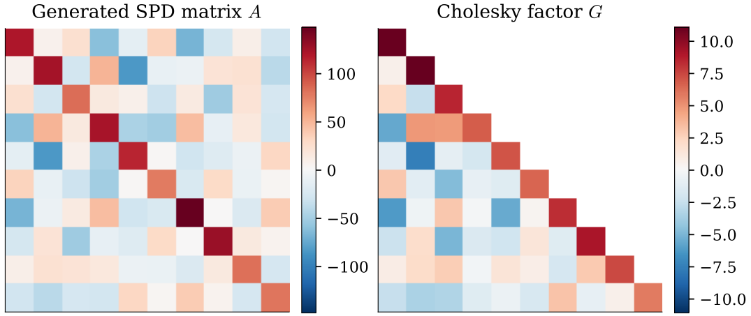
Figure 1: Structure of the generated symmetric positive-definite matrix A and its lower-triangular Cholesky factor G .
