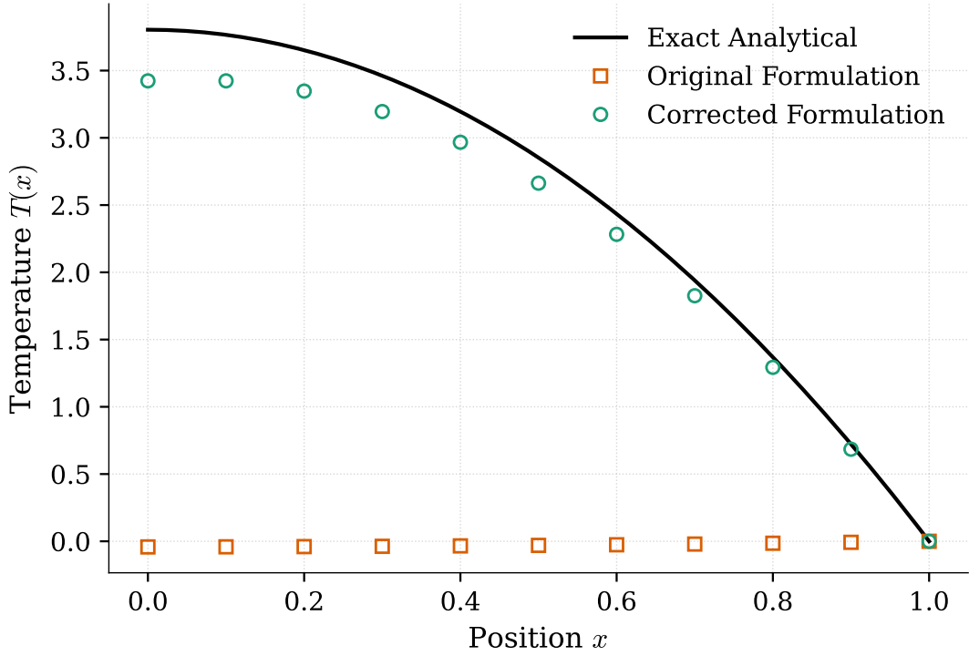
Figure 3: Comparison of the analytical solution with the profiles obtained from the original and corrected finite-difference formulations.
