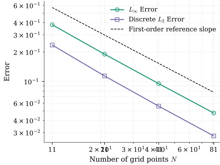
Figure 4: Observed convergence of the corrected formulation under grid refinement; the dashed line denotes a first-order reference slope.
