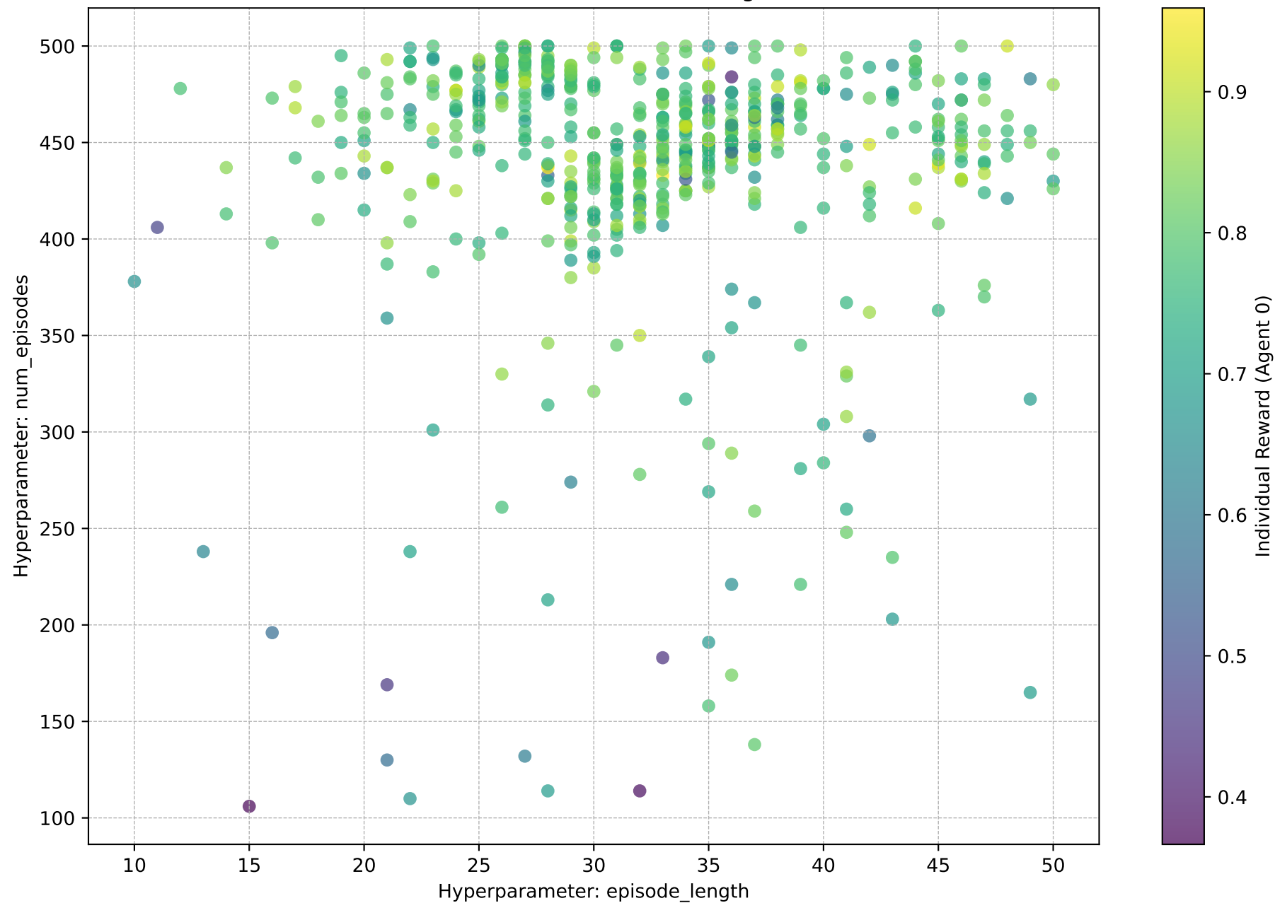
episode_length vs. num_episodes (Color shows Individual Reward (Agent 0))
