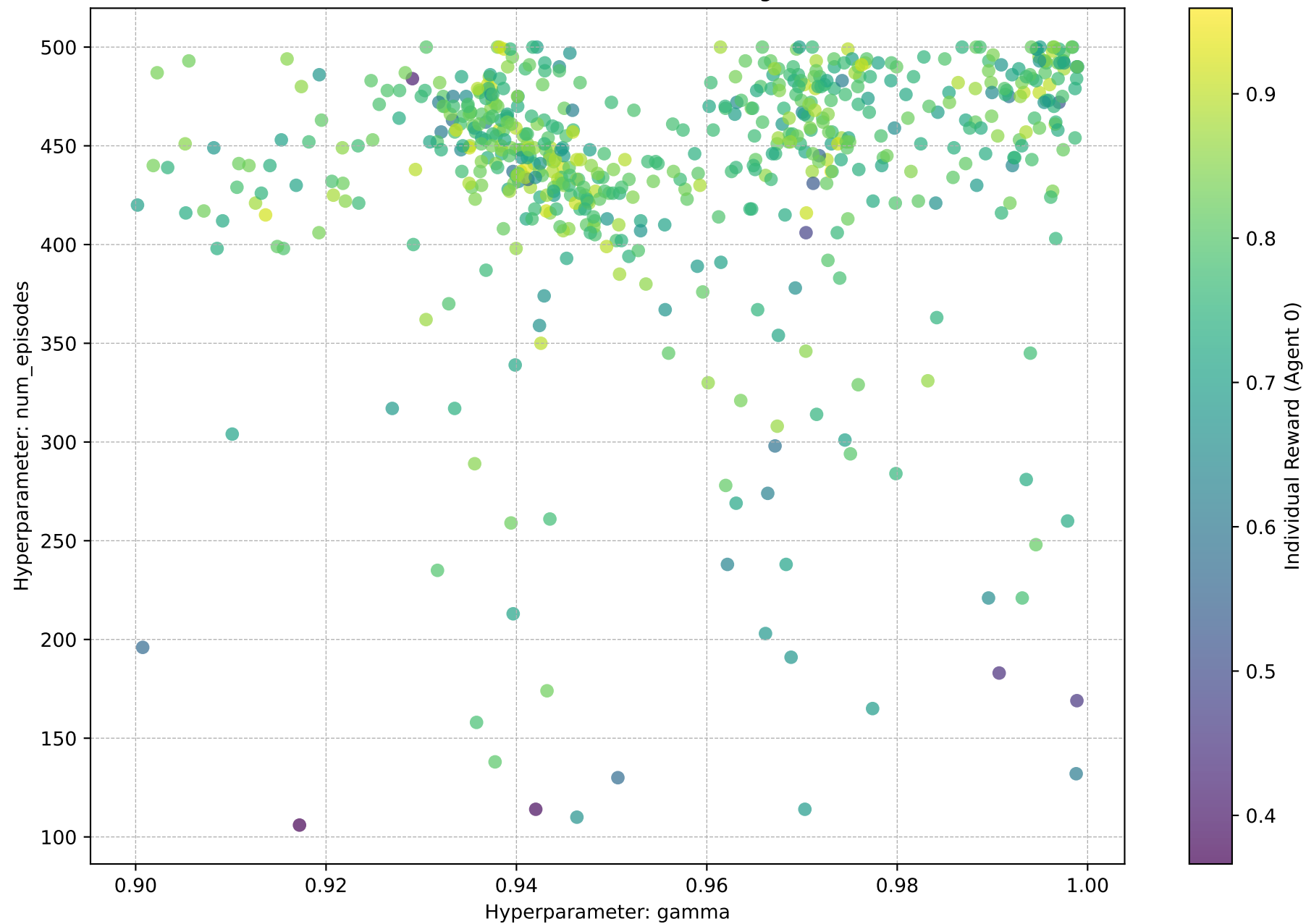
gamma vs. num_episodes (Color shows Individual Reward (Agent 0))
