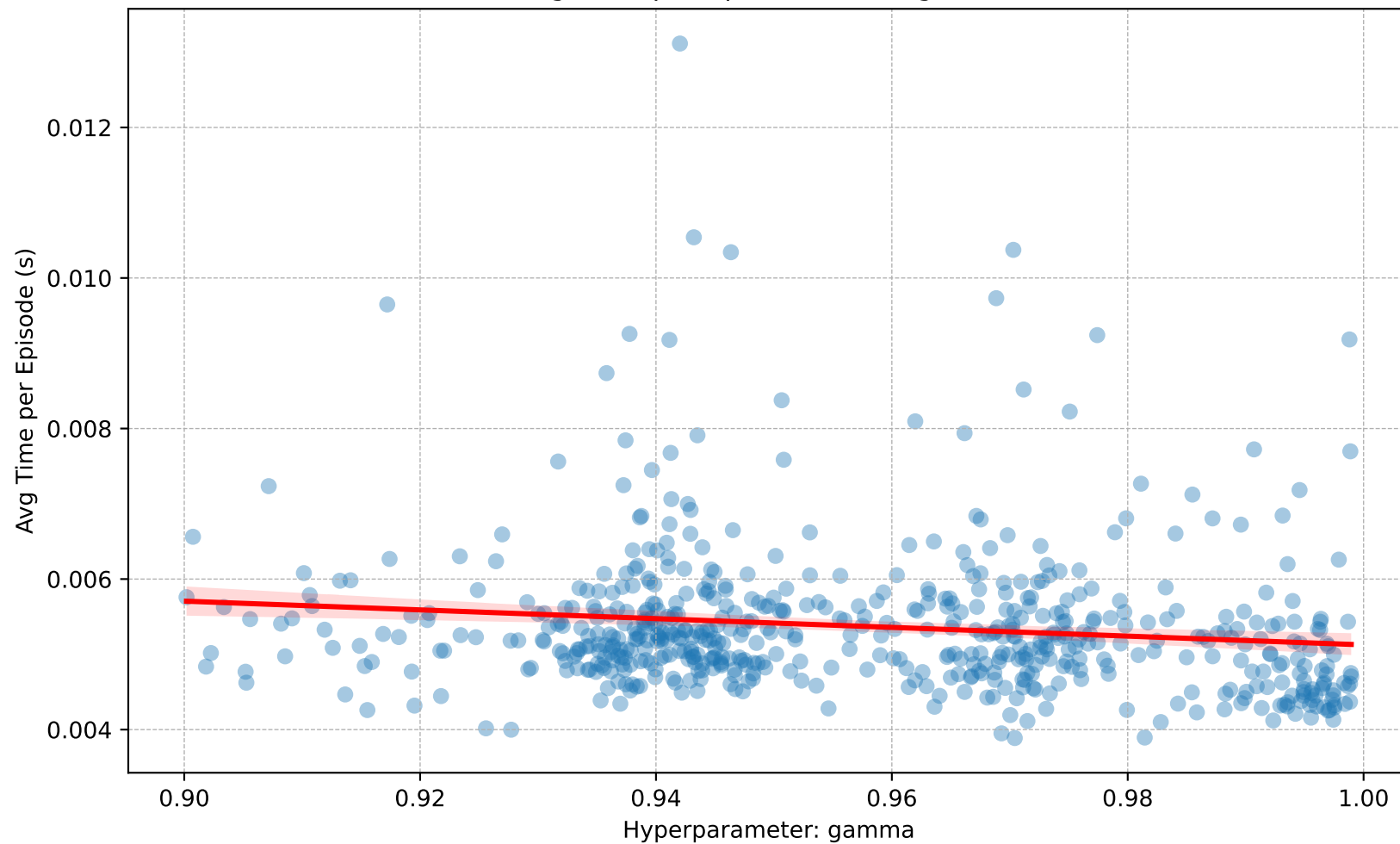
Avg Time per Episode (s) vs. gamma
