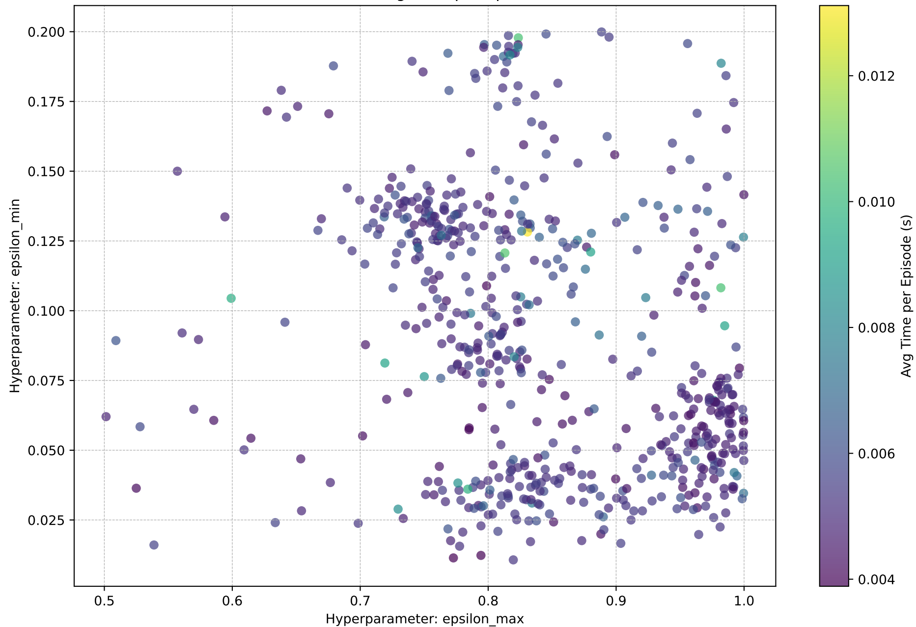
epsilon_max vs. epsilon_min (Color shows Avg Time per Episode (s))
