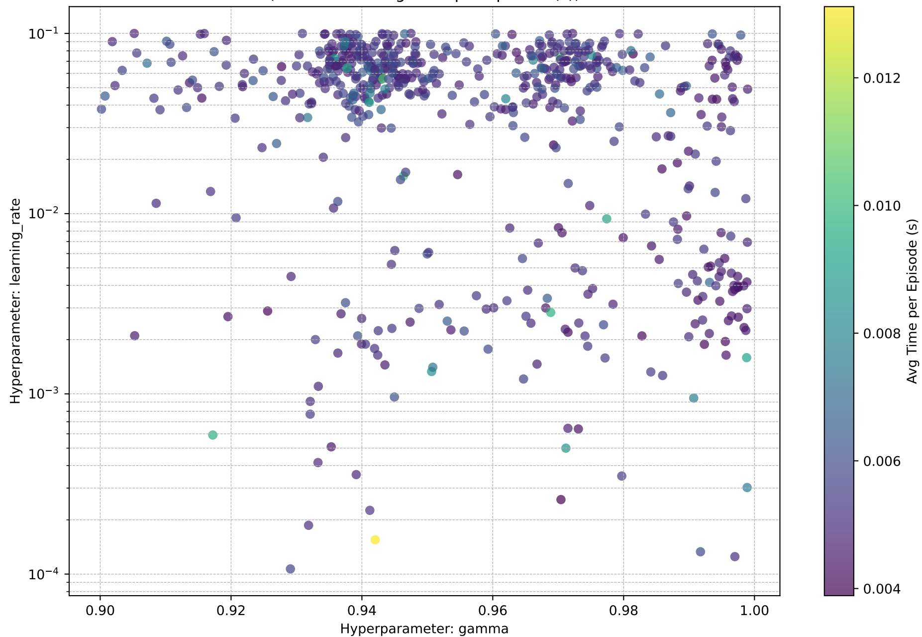
gamma vs. learning_rate (Color shows Avg Time per Episode (s))
