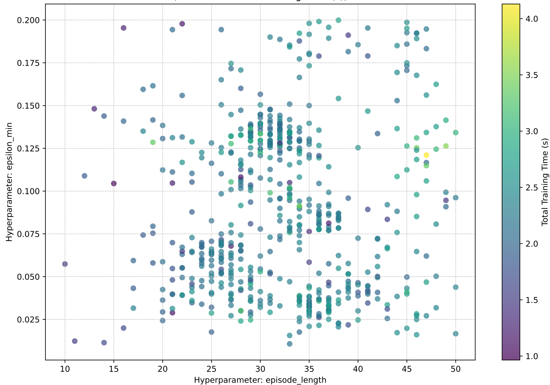
episode_length vs. epsilon_min (Color shows Total Training Time (s))
