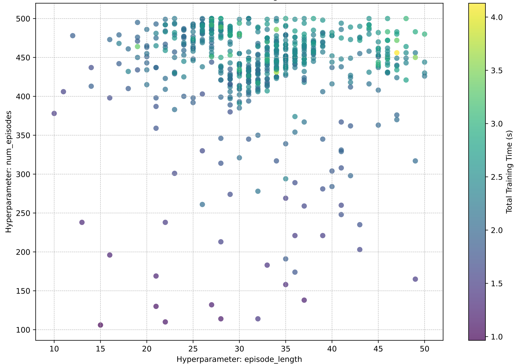
episode_length vs. num_episodes (Color shows Total Training Time (s))
