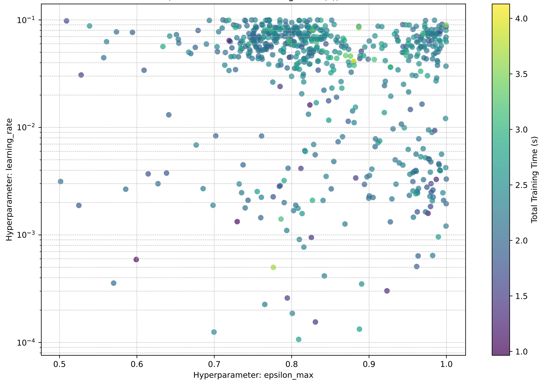
epsilon_max vs. learning_rate (Color shows Total Training Time (s))
