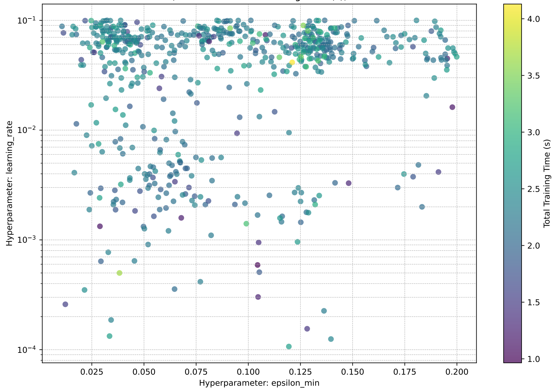
epsilon_min vs. learning_rate (Color shows Total Training Time (s))
