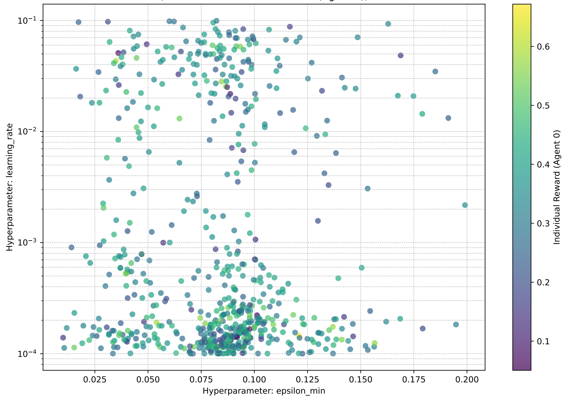
epsilon_min vs. learning_rate (Color shows Individual Reward (Agent 0))
