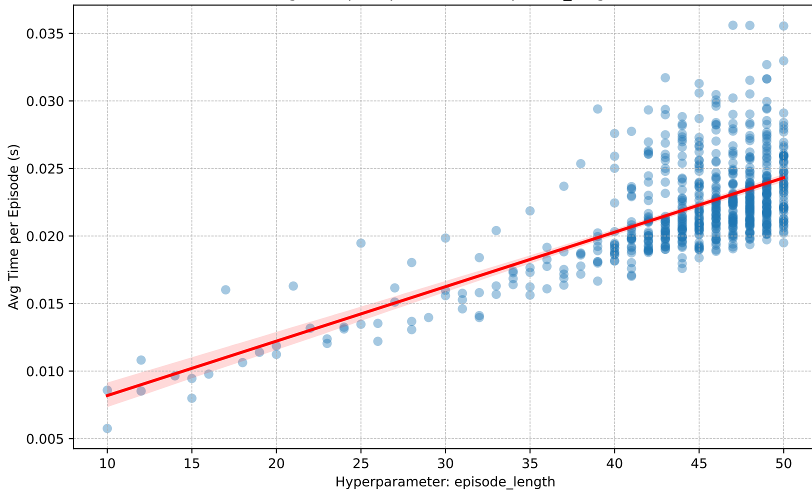
Avg Time per Episode (s) vs. episode_length
