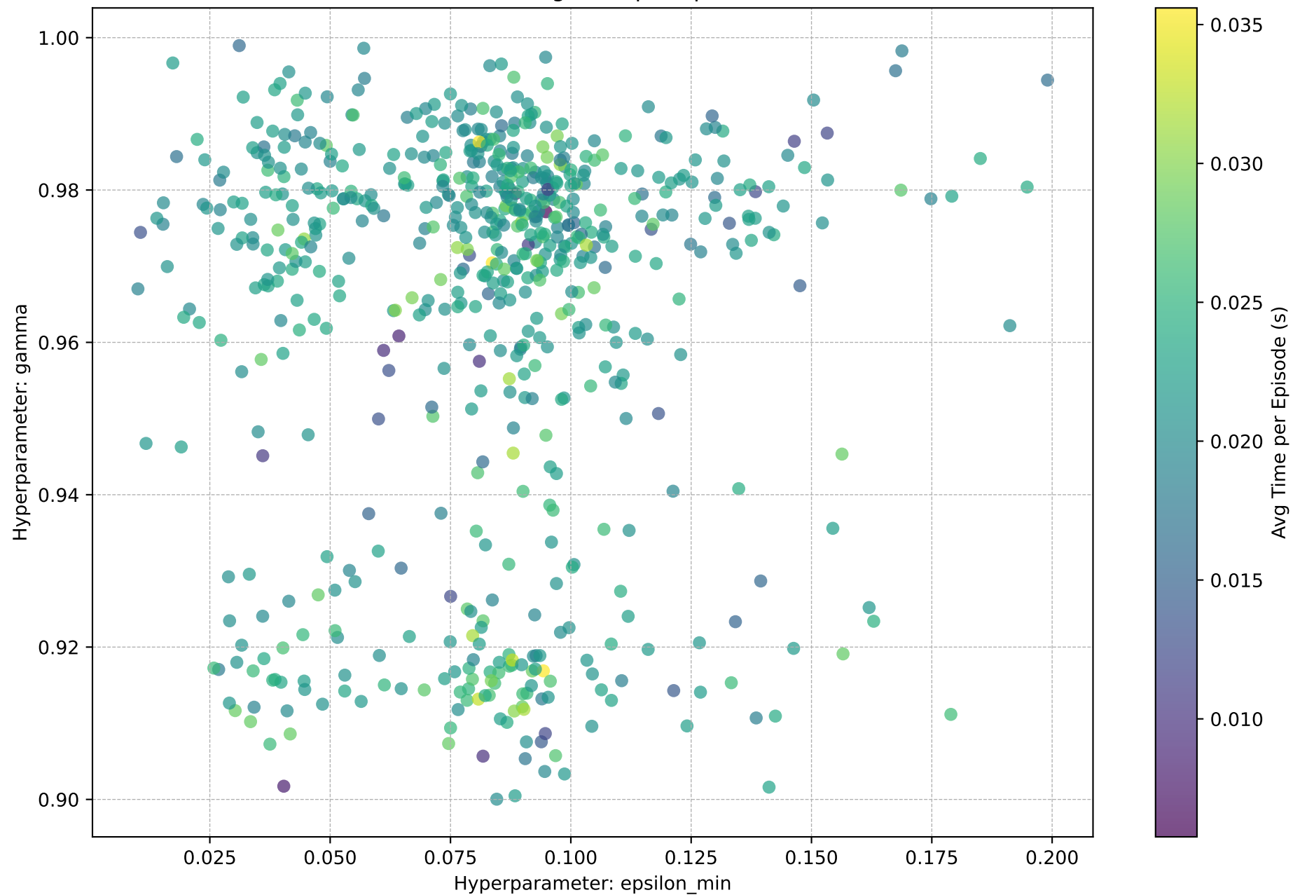
epsilon_min vs. gamma (Color shows Avg Time per Episode (s))
