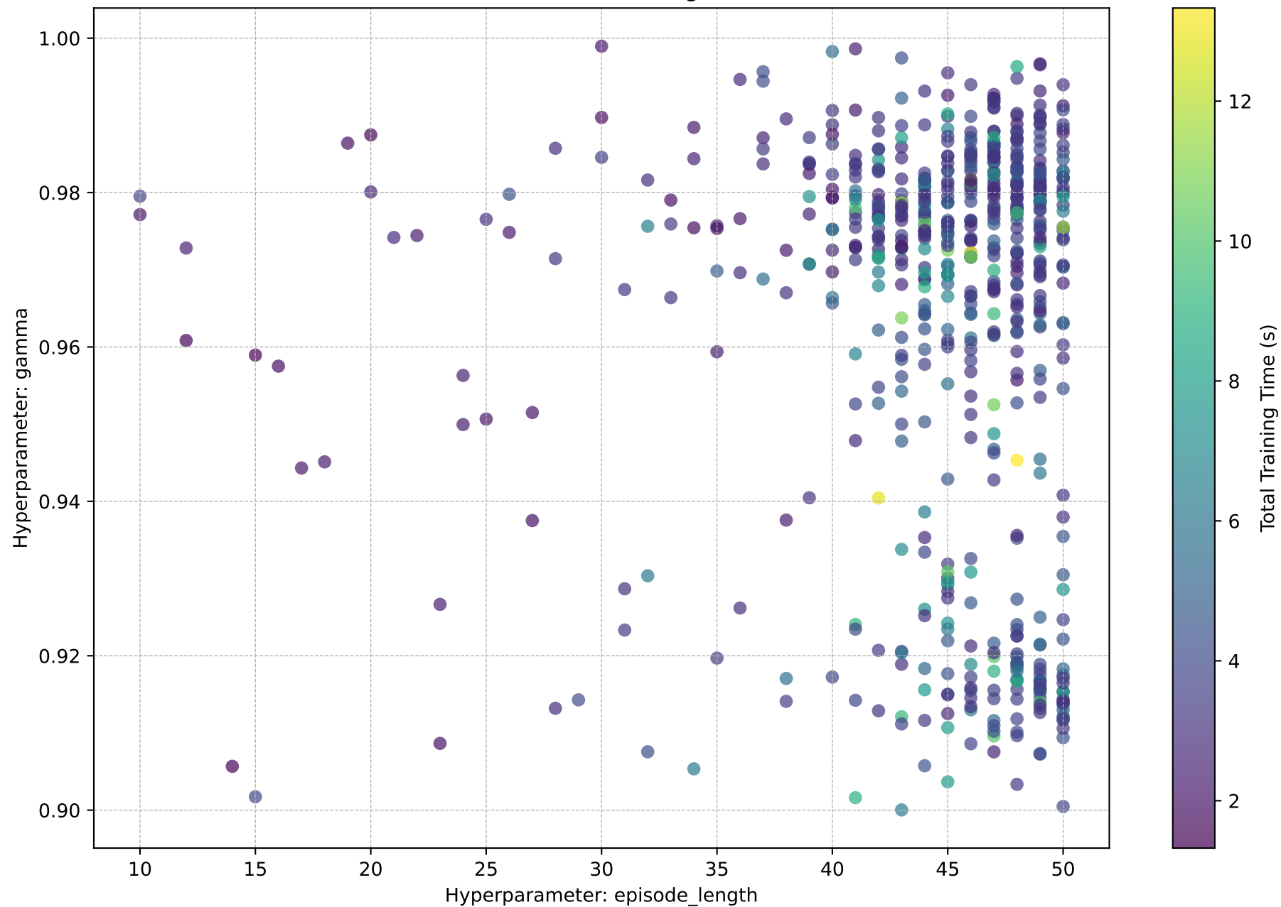
episode_length vs. gamma (Color shows Total Training Time (s))
