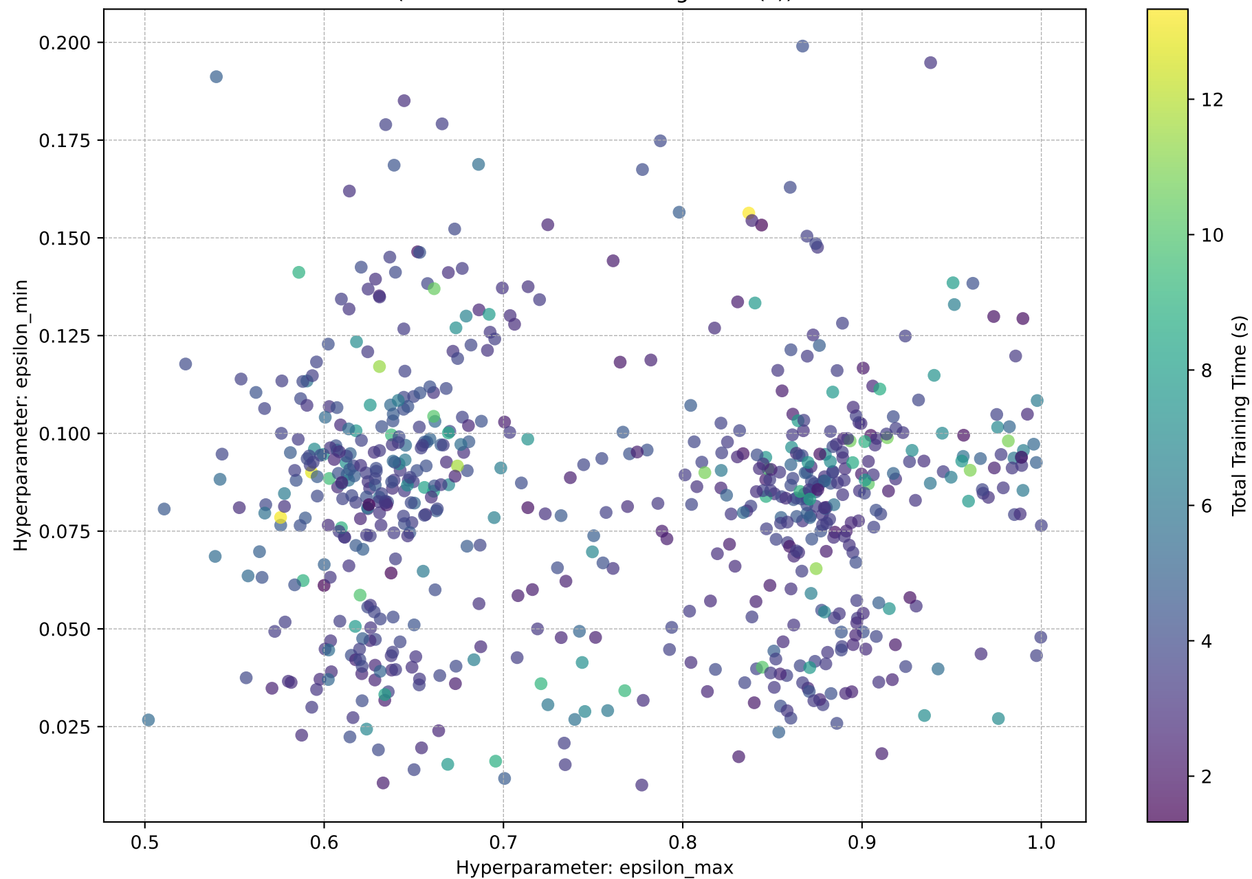
epsilon_max vs. epsilon_min (Color shows Total Training Time (s))
