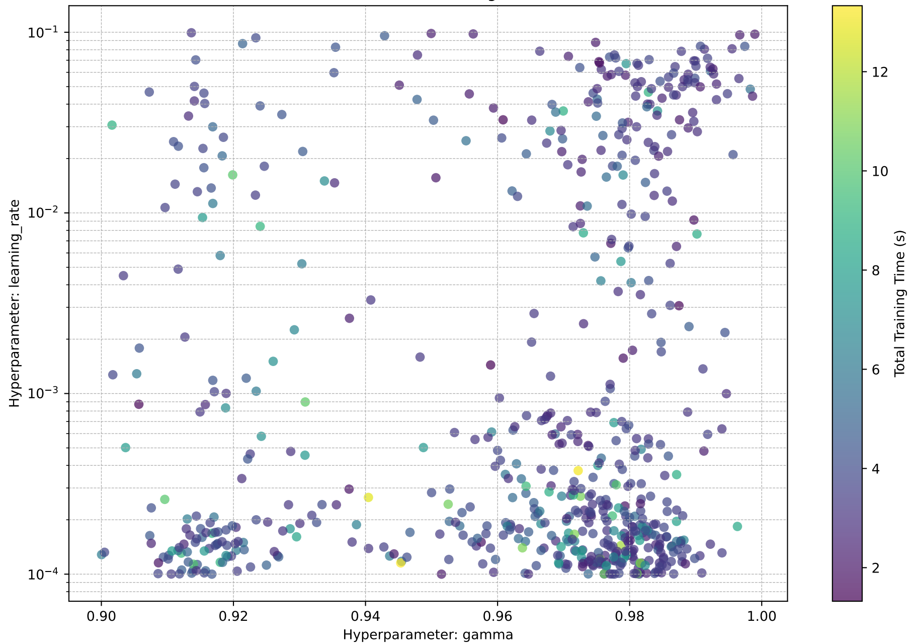
gamma vs. learning_rate (Color shows Total Training Time (s))
