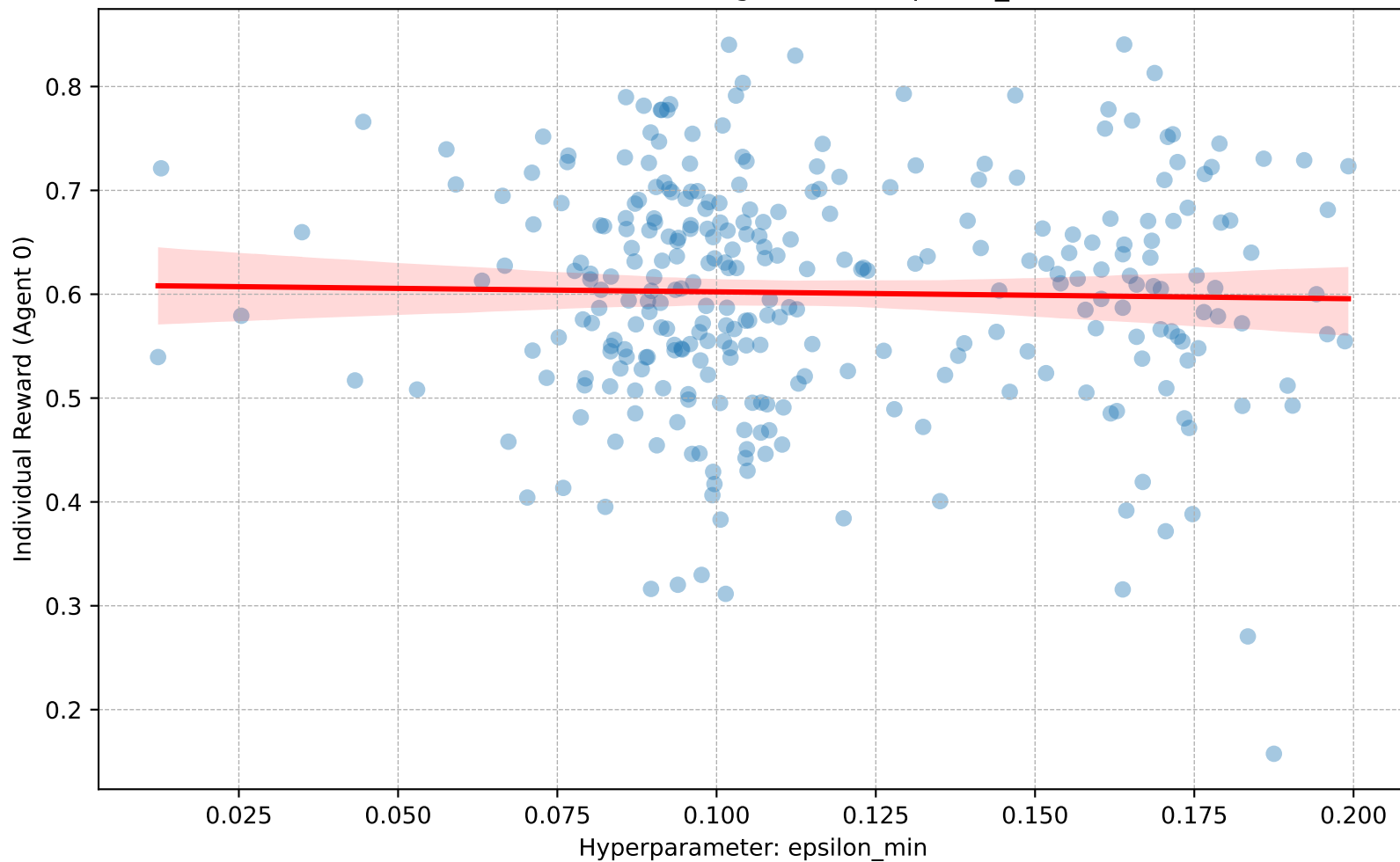
Individual Reward (Agent 0) vs. epsilon_min
