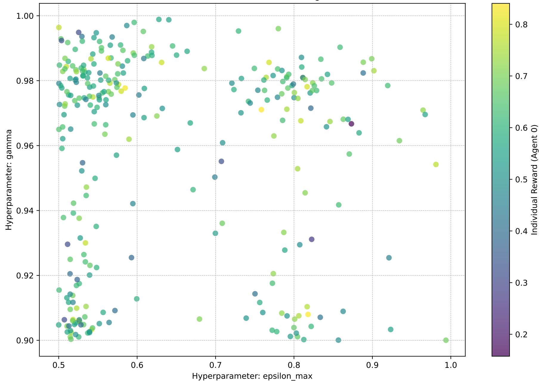
epsilon_max vs. gamma (Color shows Individual Reward (Agent 0))
