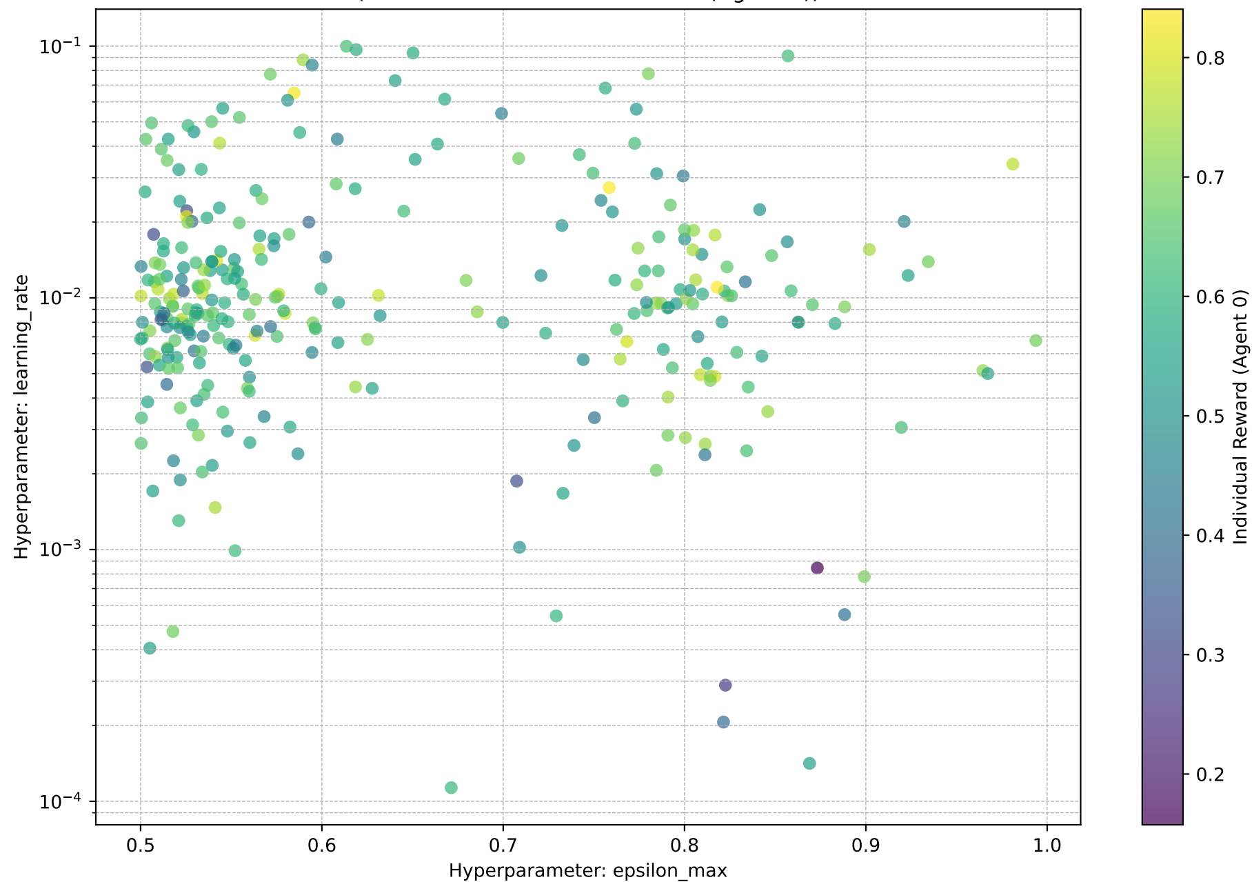
epsilon_max vs. learning_rate (Color shows Individual Reward (Agent 0))
