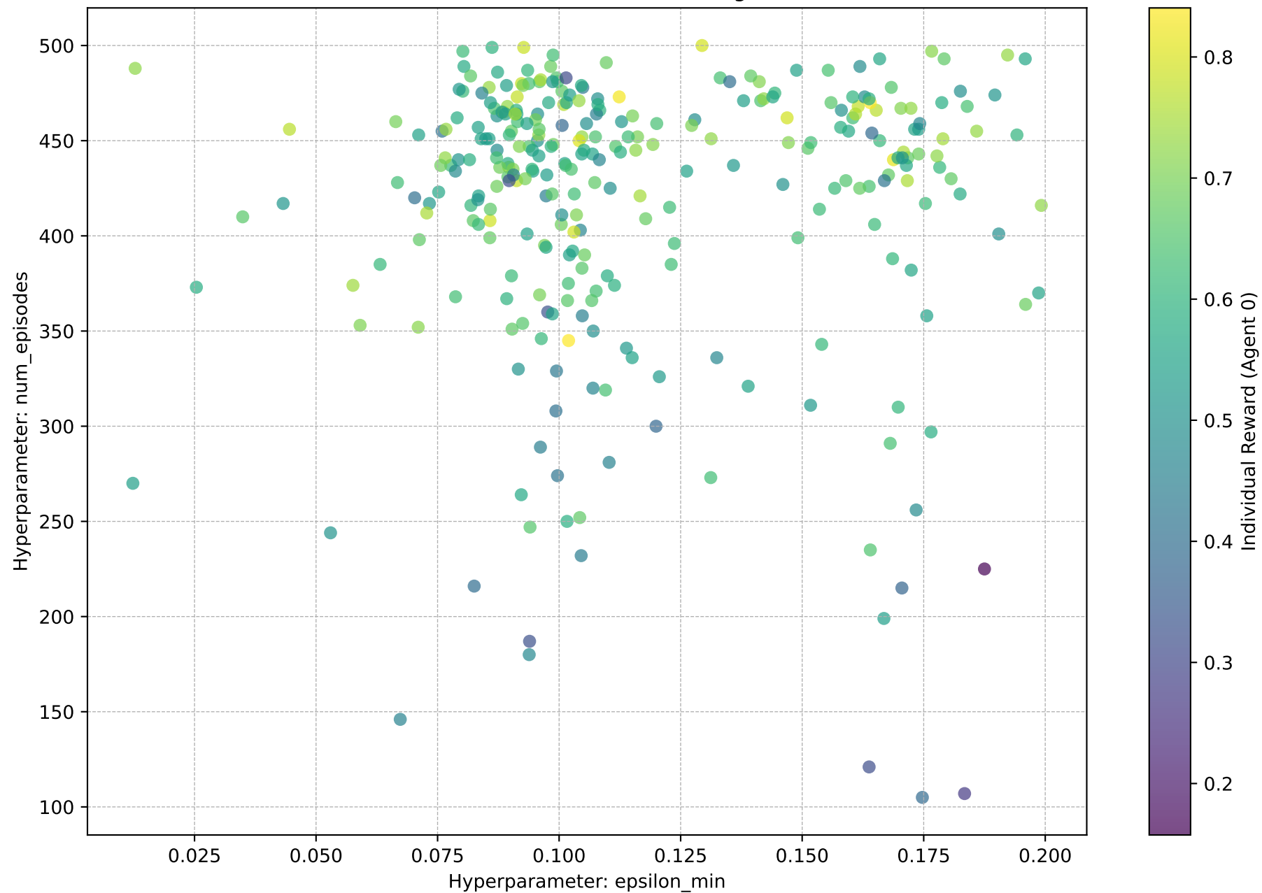
epsilon_min vs. num_episodes (Color shows Individual Reward (Agent 0))
