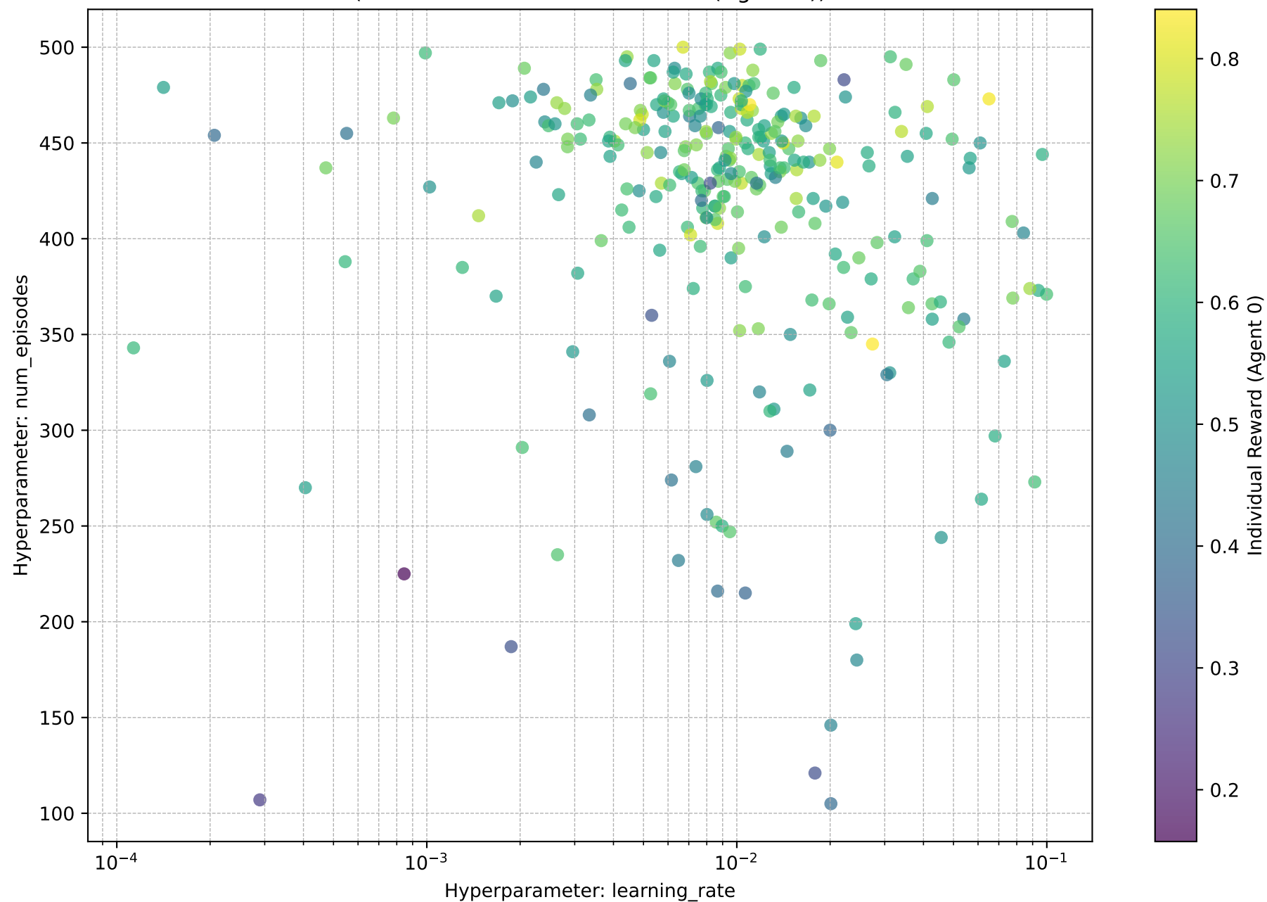
learning_rate vs. num_episodes (Color shows Individual Reward (Agent 0))
