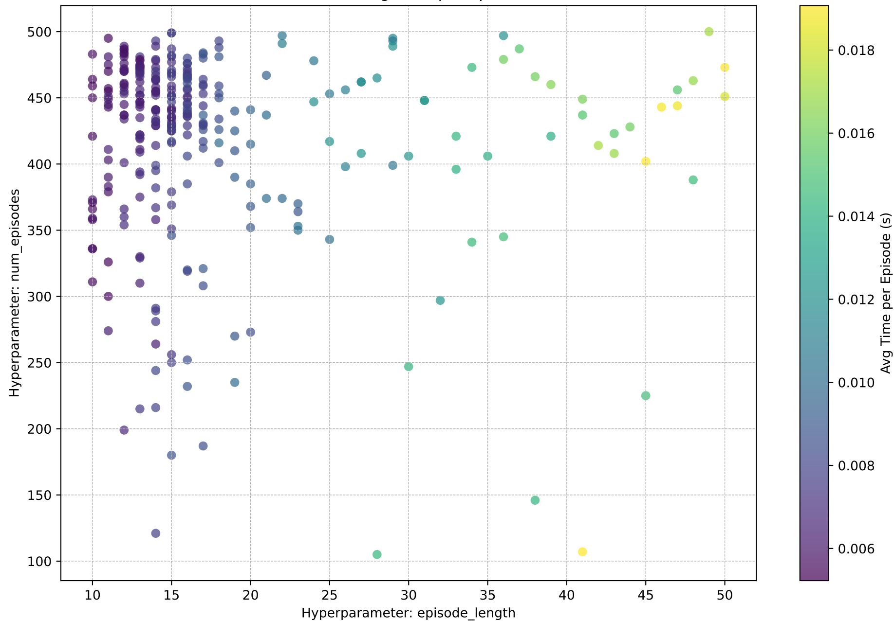
episode_length vs. num_episodes (Color shows Avg Time per Episode (s))
