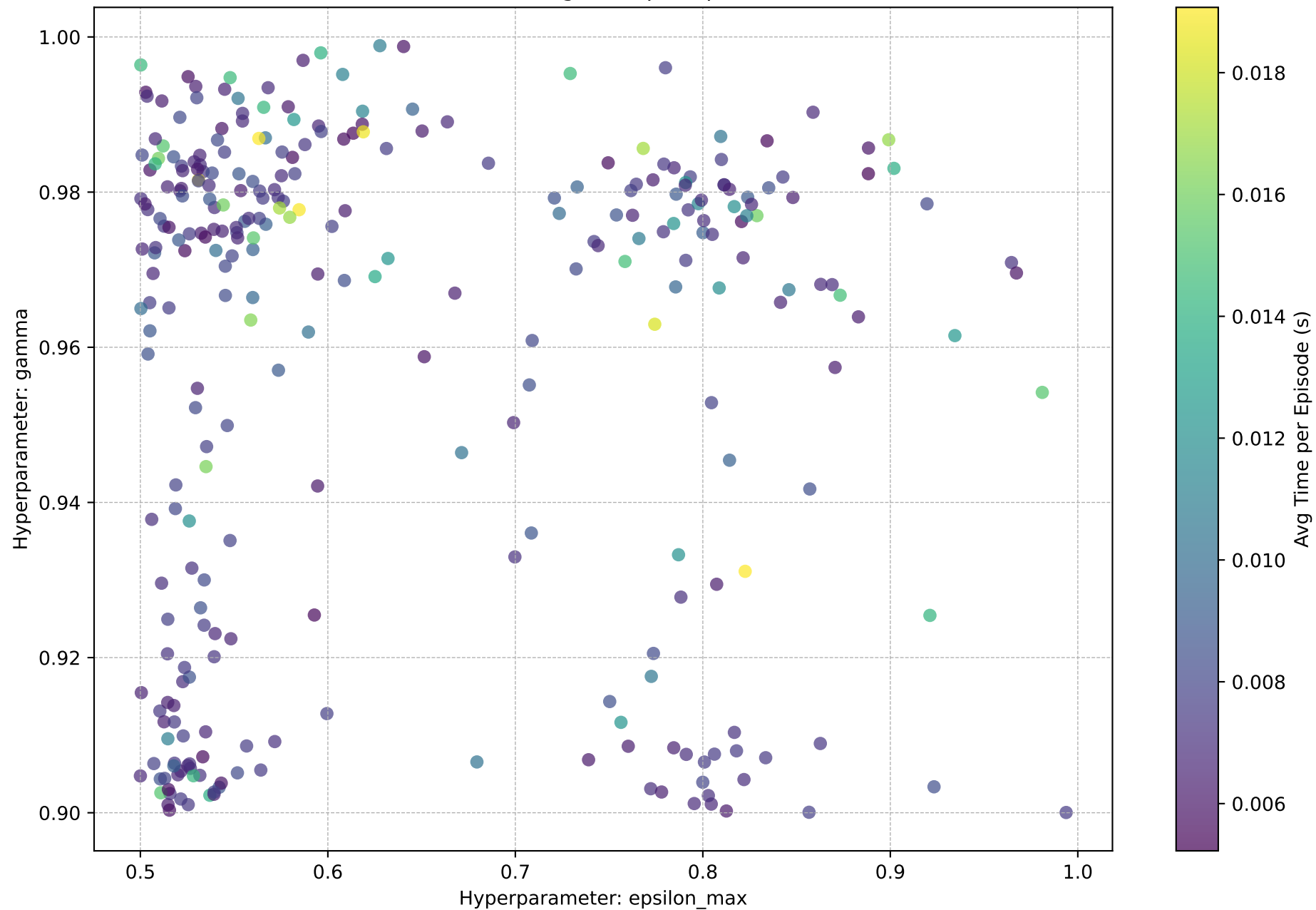
epsilon_max vs. gamma (Color shows Avg Time per Episode (s))
