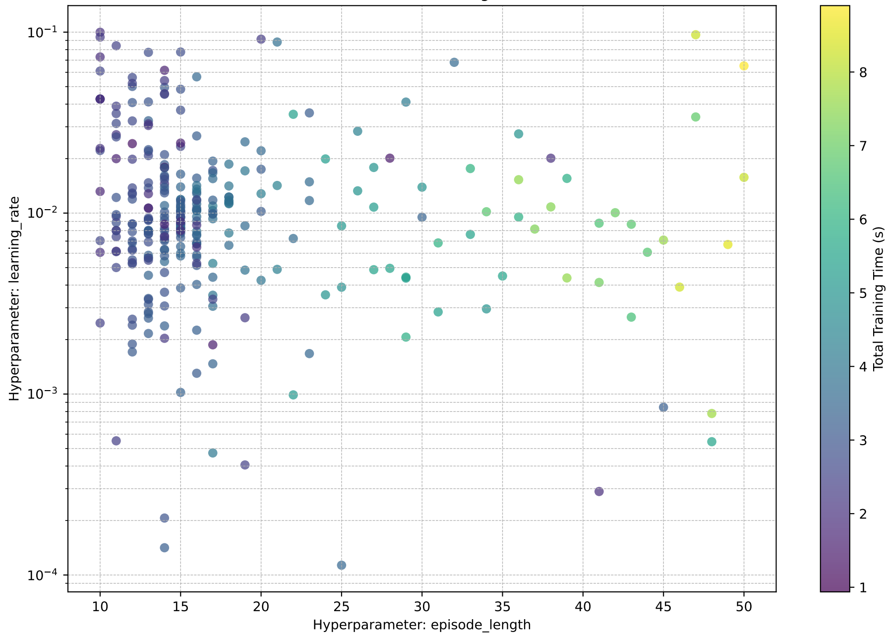
episode_length vs. learning_rate (Color shows Total Training Time (s))
