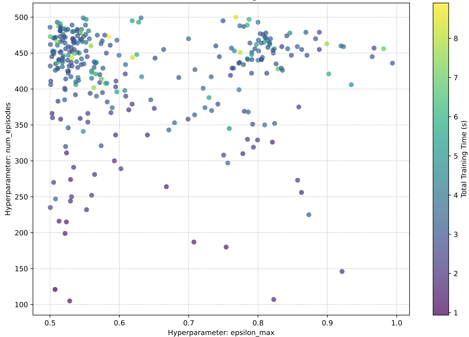
epsilon_max vs. num_episodes (Color shows Total Training Time (s))
