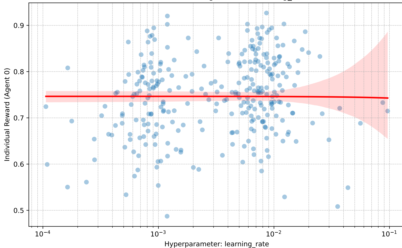
Individual Reward (Agent 0) vs. learning_rate
