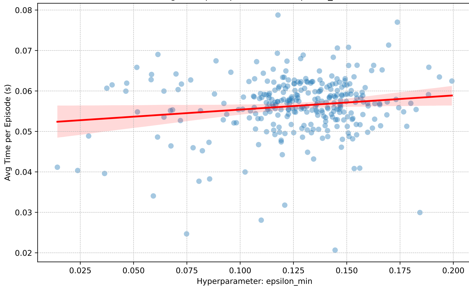
Avg Time per Episode (s) vs. epsilon_min
