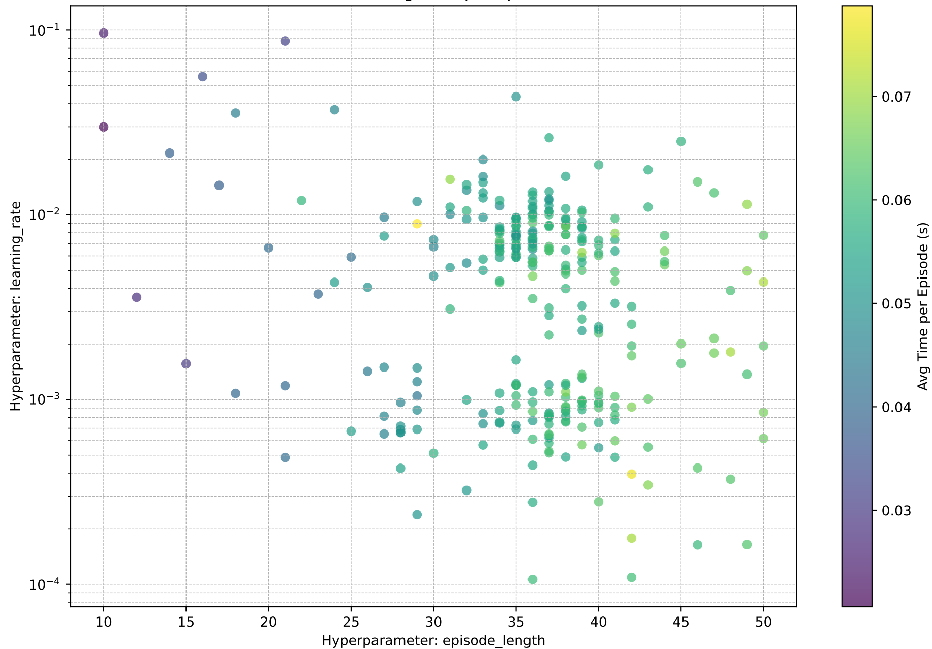
episode_length vs. learning_rate (Color shows Avg Time per Episode (s))
