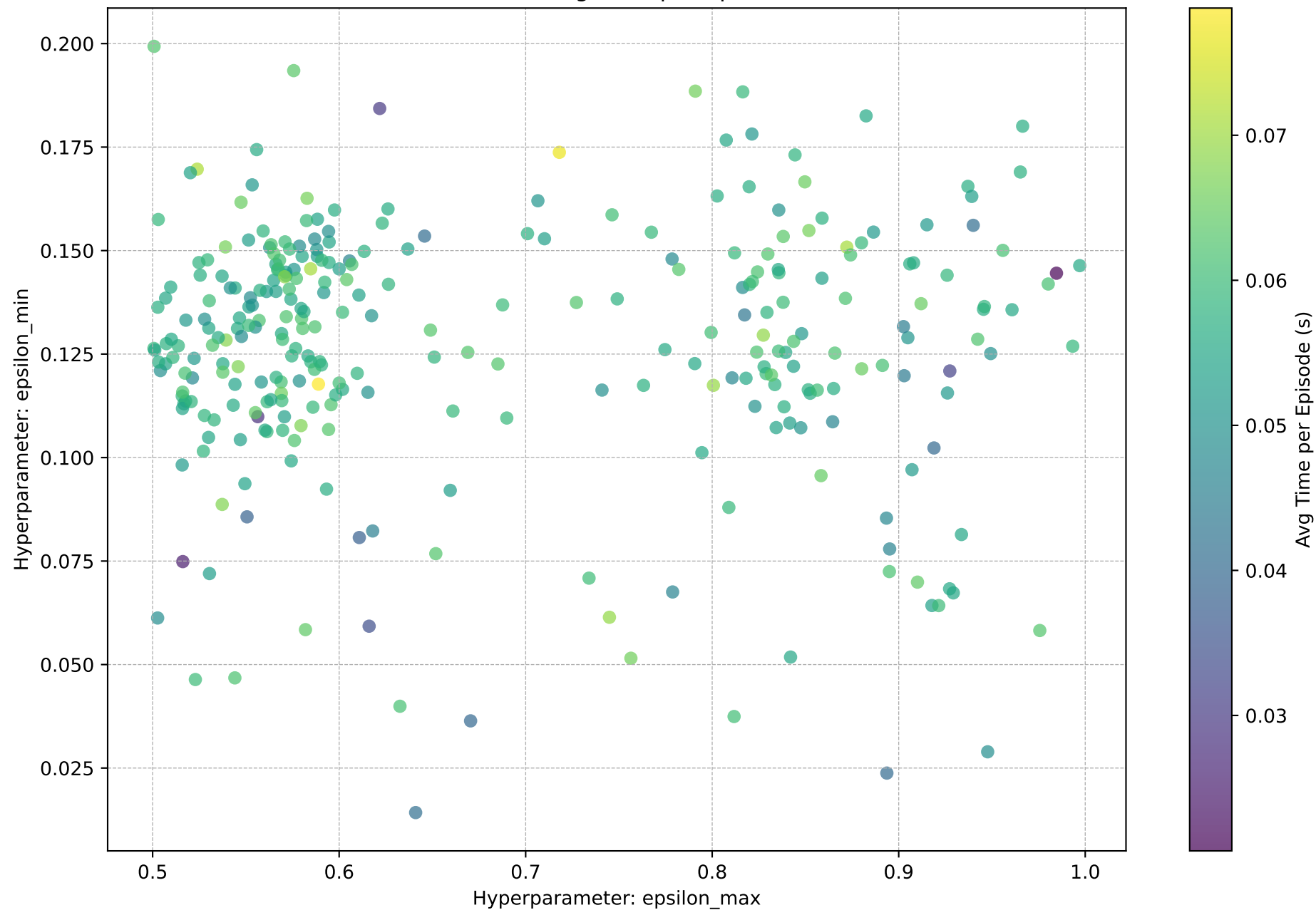
epsilon_max vs. epsilon_min (Color shows Avg Time per Episode (s))
