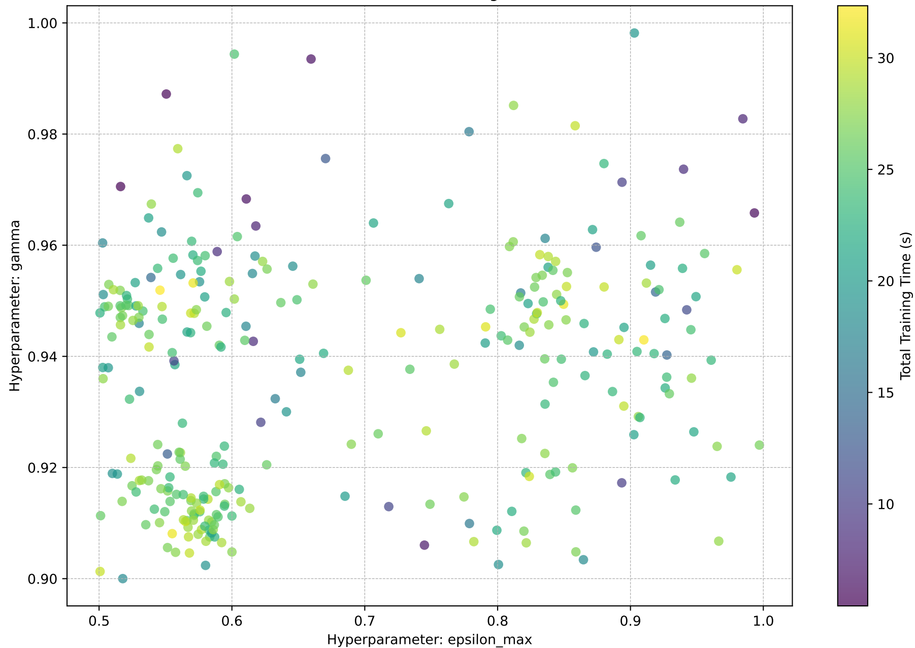
epsilon_max vs. gamma (Color shows Total Training Time (s))
