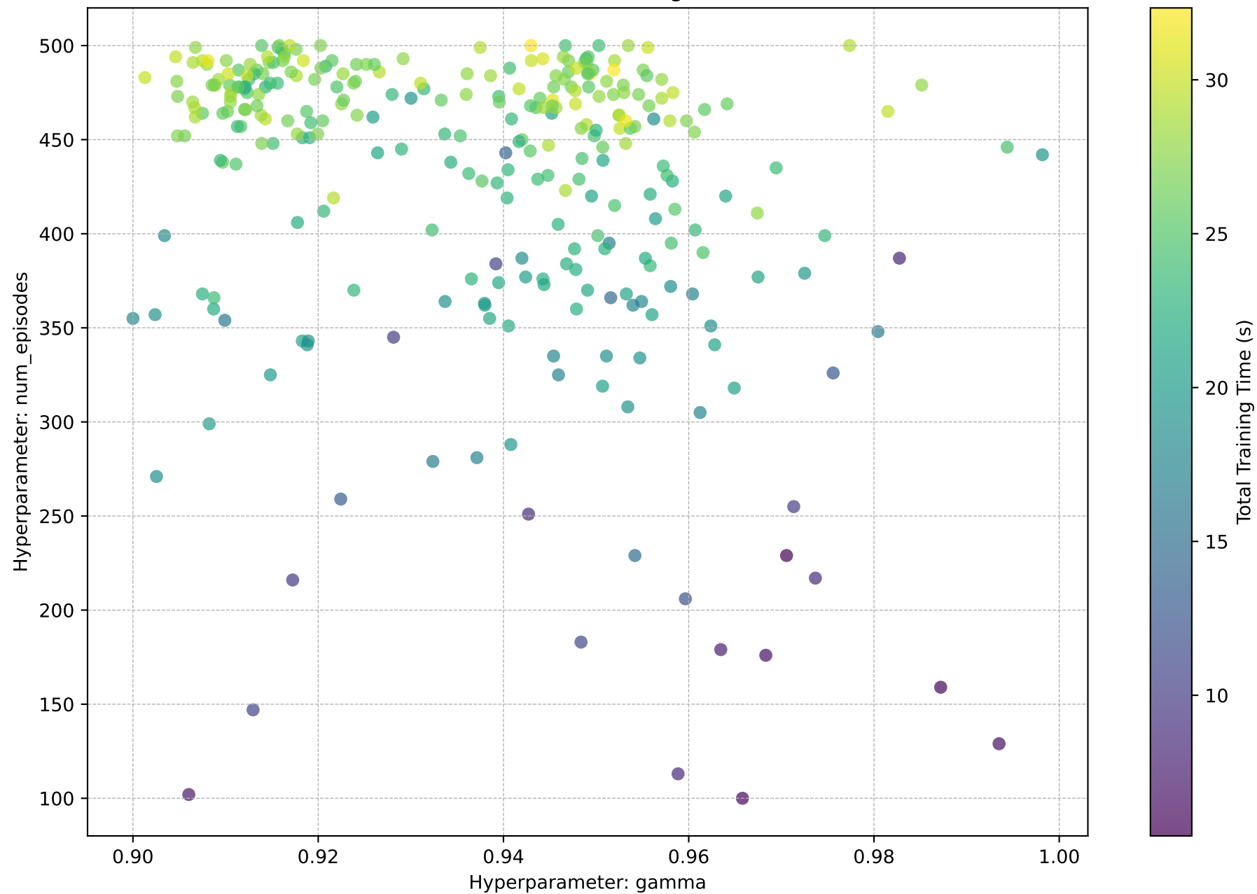
gamma vs. num_episodes (Color shows Total Training Time (s))
