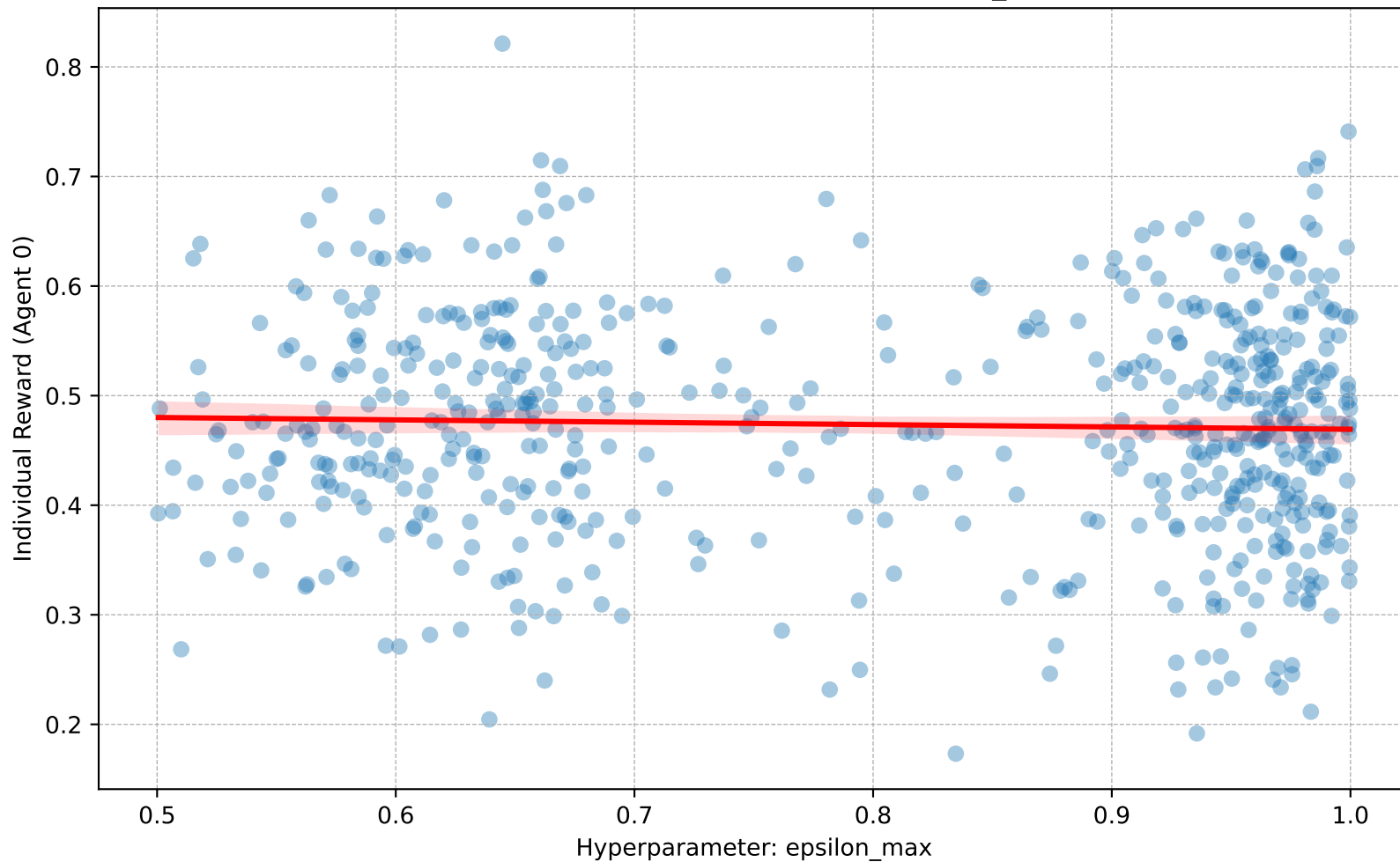
Individual Reward (Agent 0) vs. epsilon_max
